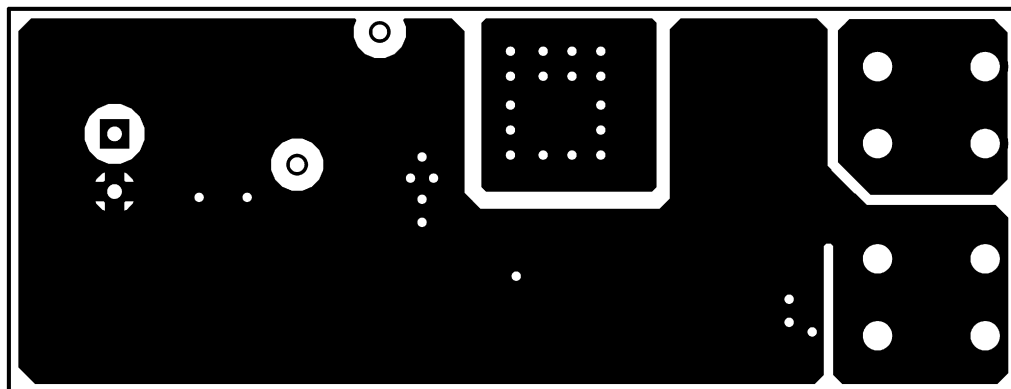
Figure 15. Solder Side
