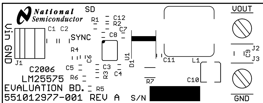
Figure 16. Silkscreen
