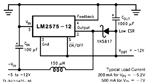
FIGURE 11. Negative Boost
