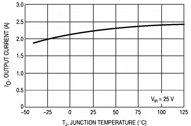
Figure 5. Current Limit
