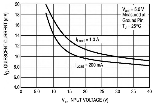
Figure 7. Quiescent Current
