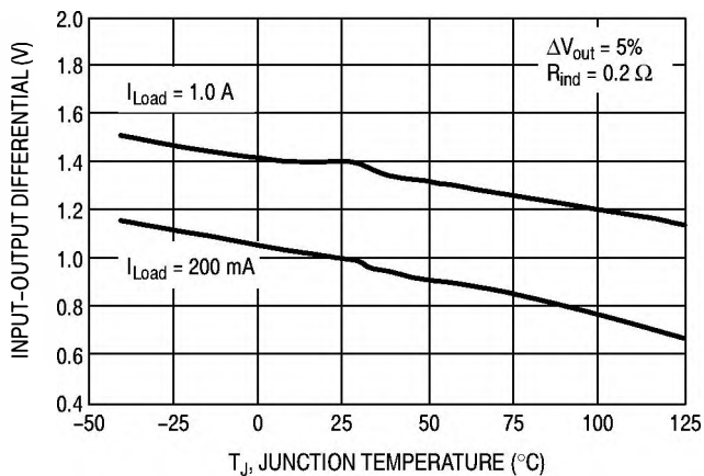
Figure 6. Dropout Voltage
