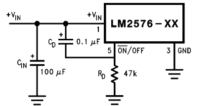
FIGURE 14. Delayed Startup
