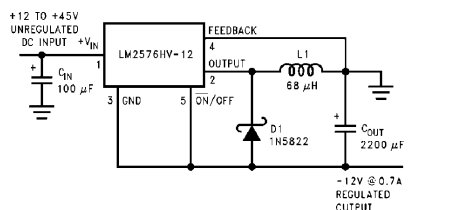
FIGURE 10. Inverting Buck-Boost Develops -12\text{V}
