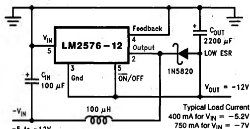
FIGURE 11. Negative Boost
