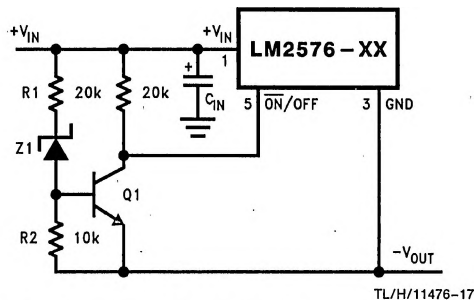
FIGURE 13. Undervoltage Lockout for Buck-Boost Circuit
