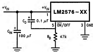
FIGURE 14. Delayed Startup
