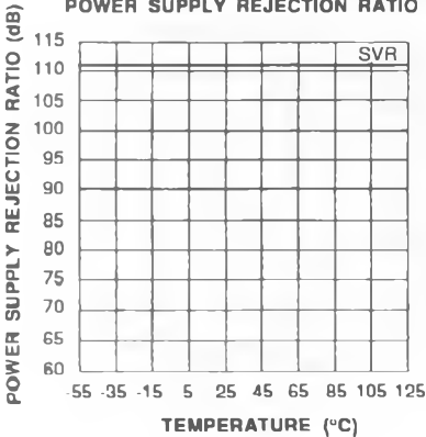
POWER SUPPLY REJECTION RATIO
