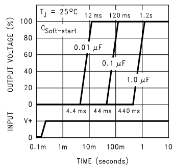
Soft-start Response
