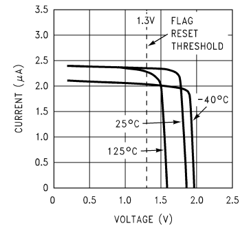
Delay Pin Current
