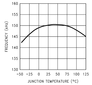
Switching Frequency
