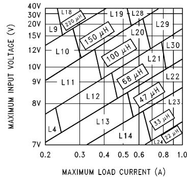
FIGURE 6. LM2595-5.0
