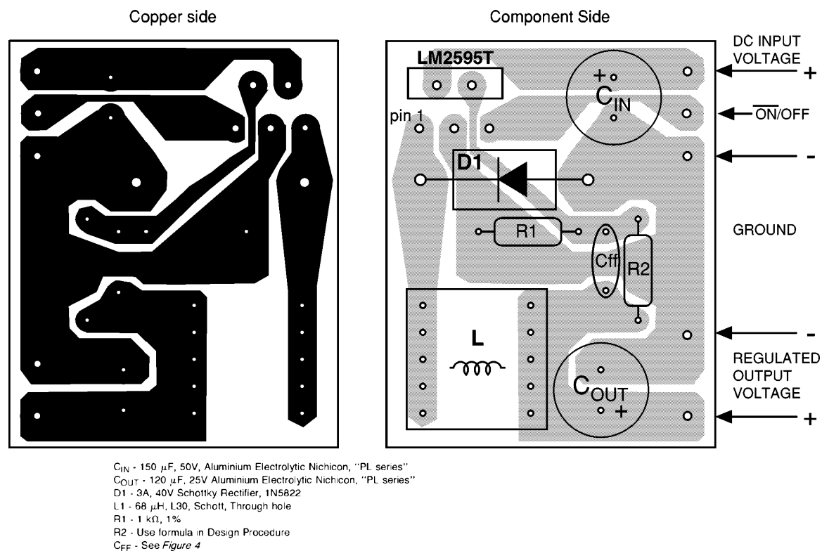
FIGURE 29. PC Board Layout (Continued)
