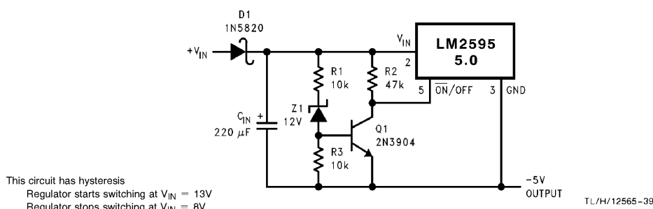
FIGURE 24. Undervoltage Lockout with Hysteresis for Inverting Regulator
