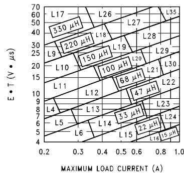
FIGURE 8. LM2595-ADJ
