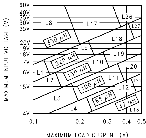
Figure 28. LM2597/LM2597HV-12
