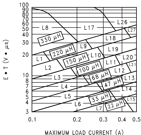
Figure 29. LM2597/LM2597HV-ADJ
