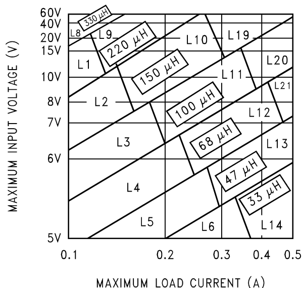
Figure 26. LM2597/LM2597HV-3.3
