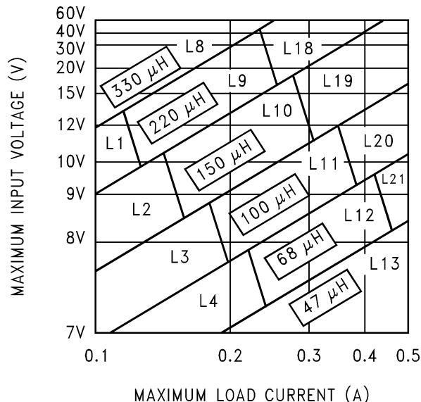
Figure 27. LM2597/LM2597HV-5.0
