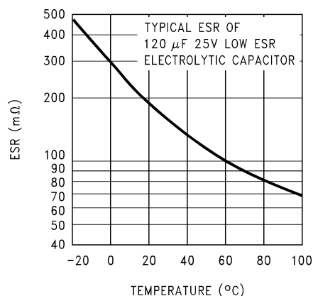
Figure 37. Capacitor ESR Change vs Temperature
