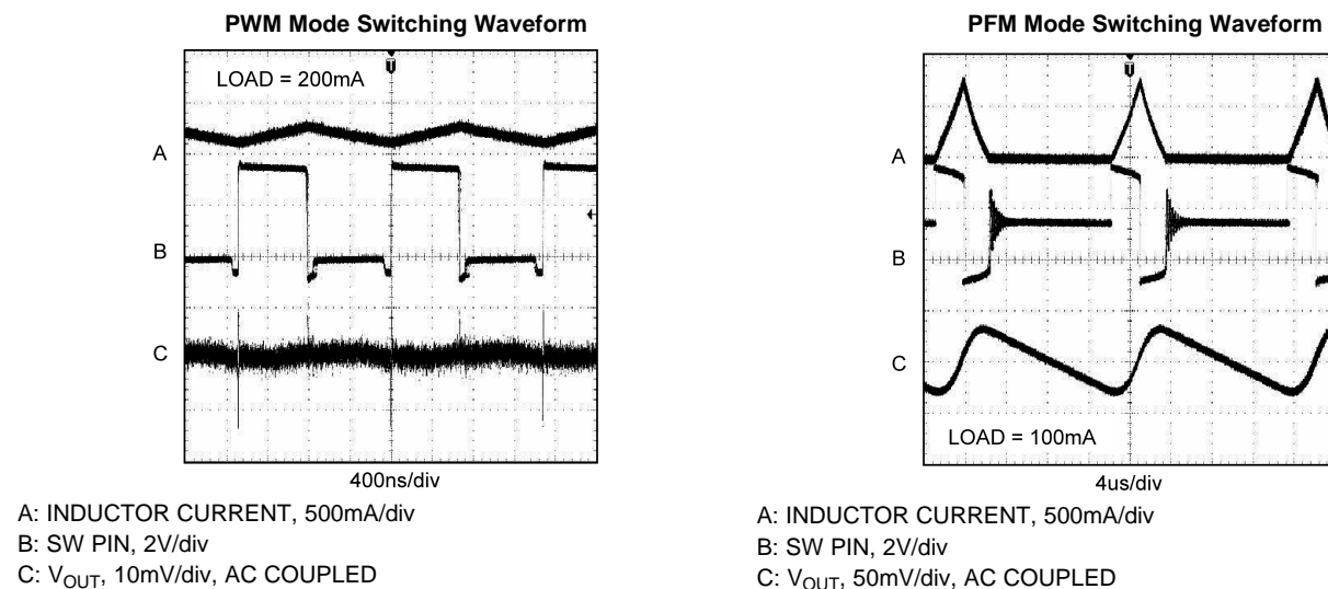
Figure 31. Typical Circuit Waveforms in (a) PWM Mode and (b) PFM Mode
