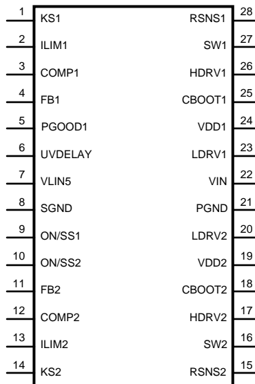
Figure 1. 28-Lead TSSOP
