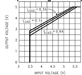
Dropout Voltage—5.0V Option
