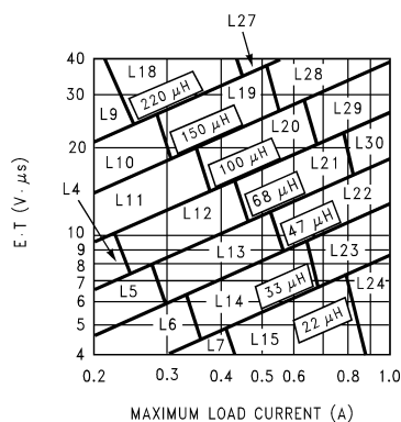
Figure 12. LM2675-ADJ
