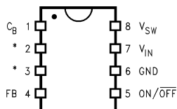
Figure 2. SO-8/DIP Package
