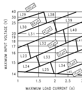
Figure 12. LM2676-12
