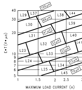
Figure 13. LM2676-ADJ
