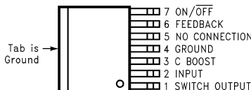
Figure 1. TO-263 Package Top View
