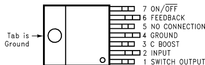
Figure 2. TO-220 Package Top View
