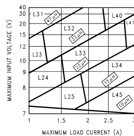
Figure 11. LM2676-5.0
