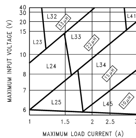
Figure 10. LM2676-3.3
