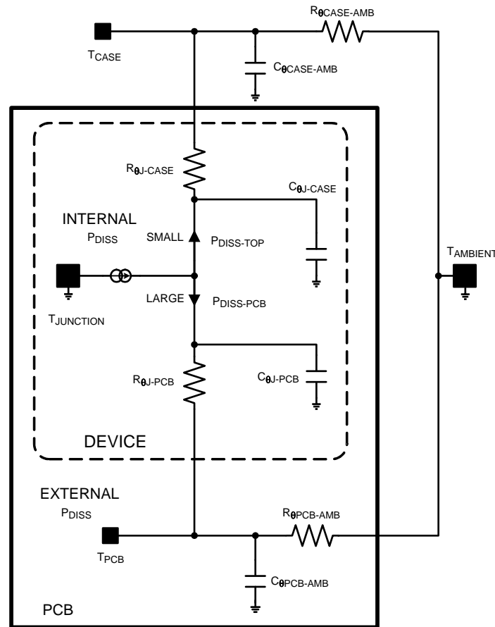
Figure 16. Associated Thermal Model
