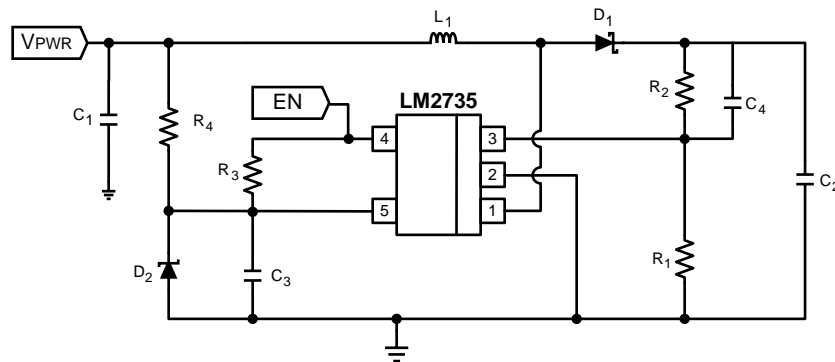
Figure 40. LM2735X (1.6MHz): V PWR = 9V, V out = 12V @ 500mA
