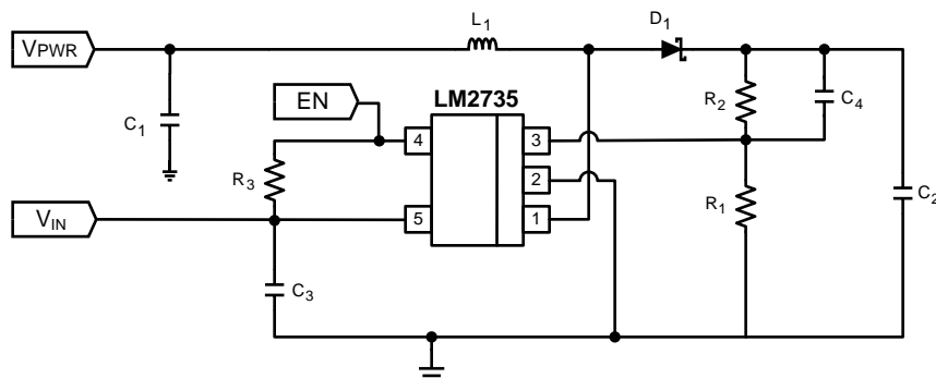
Figure 41. LM2735X (1.6MHz): V_{PWR} = 9V in = 2.7V - 5.5V, V_{out} = 12V @ 500mA
