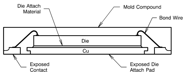
Figure 23. Internal LLP Connection
