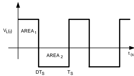
Figure 19. Inductor Volt-Sec Balance Waveform
