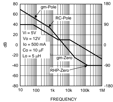
Figure 10. LM2735 Without External Compensation
