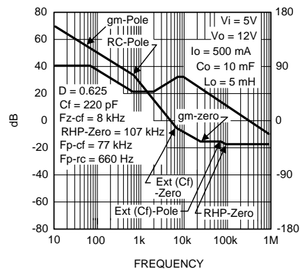
Figure 11. LM2735 With External Compensation
