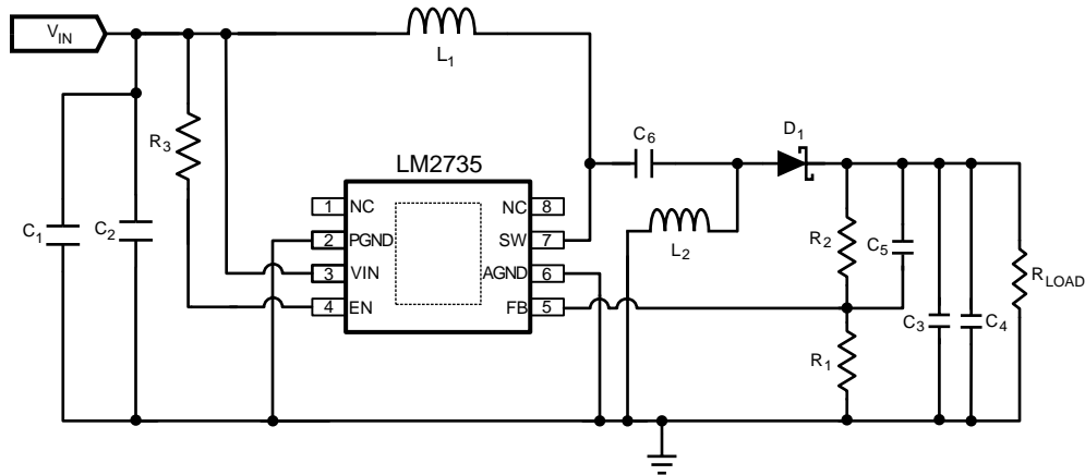
Figure 37. LM2735Y (520kHz): V_{in} = 2.7V - 5V , V_{out} = 3.3V @ 500mA
