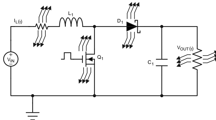
Figure 15. Thermal Schematic
