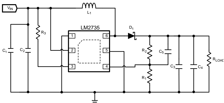
Figure 34. LM2735X (1.6MHz): V_{in} = 3.3V , V_{out} = 20V @ 150mA
