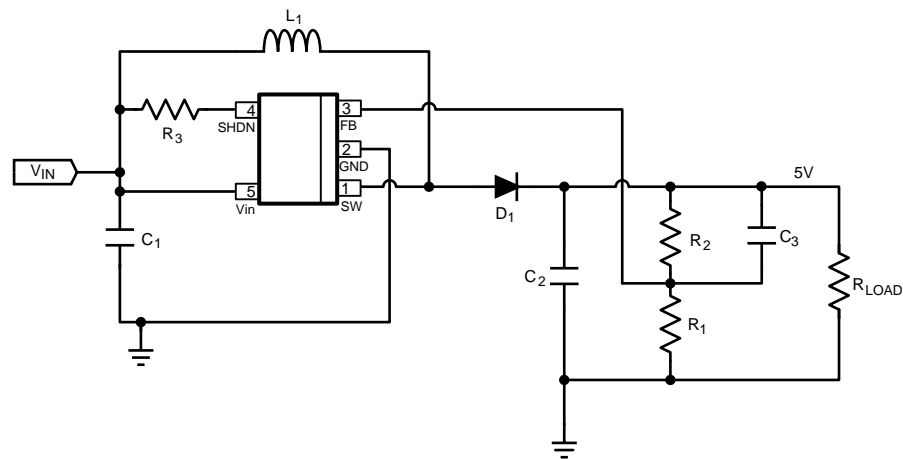
Figure 30. LM2735X (1.6MHz): V in = 3V, V out = 5V @ 500mA
