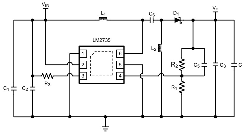
Figure 36. LM2735X (1.6MHz): Vin = 2.7V - 5V, Vout = 3.3V @ 500mA
