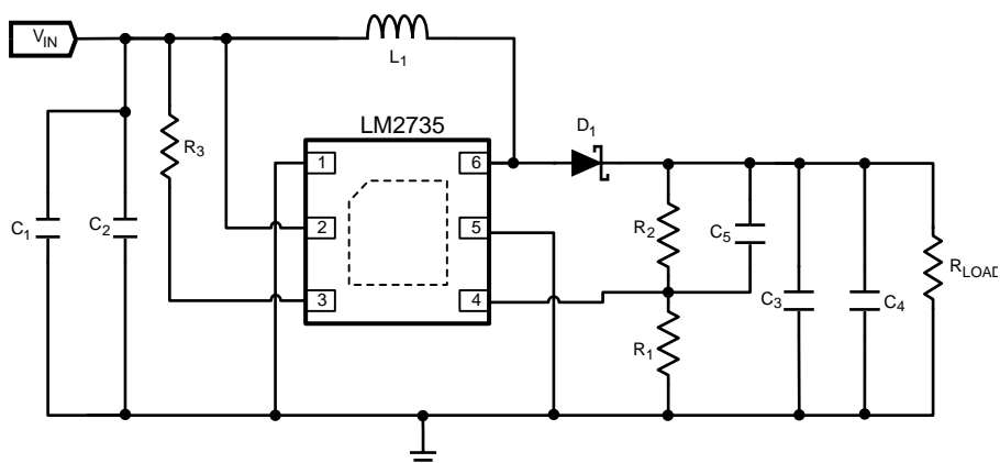
Figure 35. LM2735Y (520kHz): V_{in} = 3.3V , V_{out} = 20V @ 150mA
