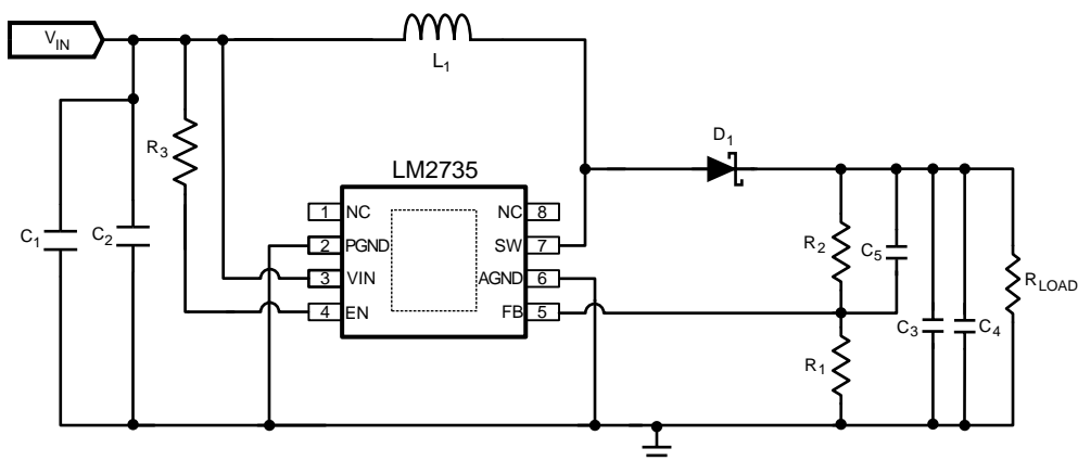
Figure 29. LM2735Y (520kHz): V_{in} = 3.3V , V_{out} = 12V @ 350mA
