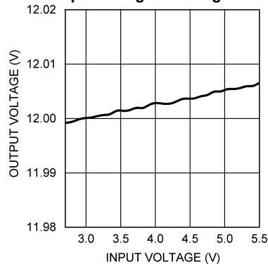
Output Voltage Line Regulation
