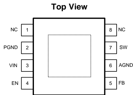
Figure 4. 8-Pin eMSOP
