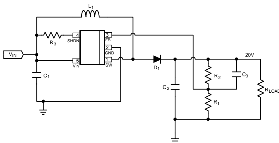
Figure 33. LM2735Y (520kHz): V in = 3.3V, V out = 20V @ 100mA
