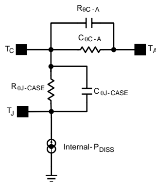
Figure 14. Simplified Thermal Impedance Model
