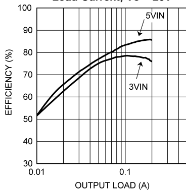
LM2735X Efficiency vs
