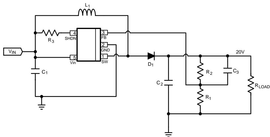
Figure 32. LM2735X (1.6MHz): V_{in} = 3.3V , V_{out} = 20V @ 100mA
