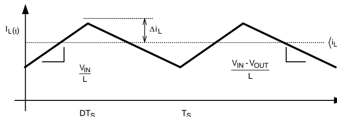
Figure 8. Inductor Current
