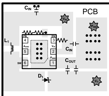
Figure 13. Example of Proper PCB Layout
