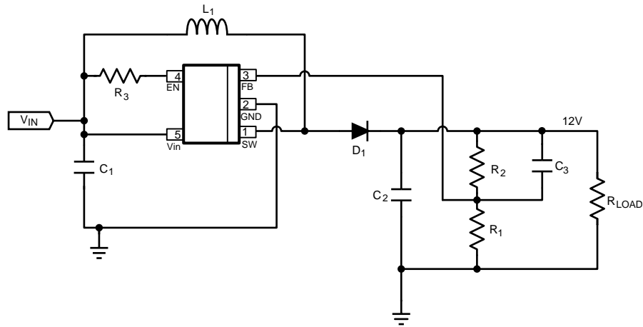
Figure 25. LM2735X (1.6MHz): V_{in} = 5V , V_{out} = 12V @ 350mA
