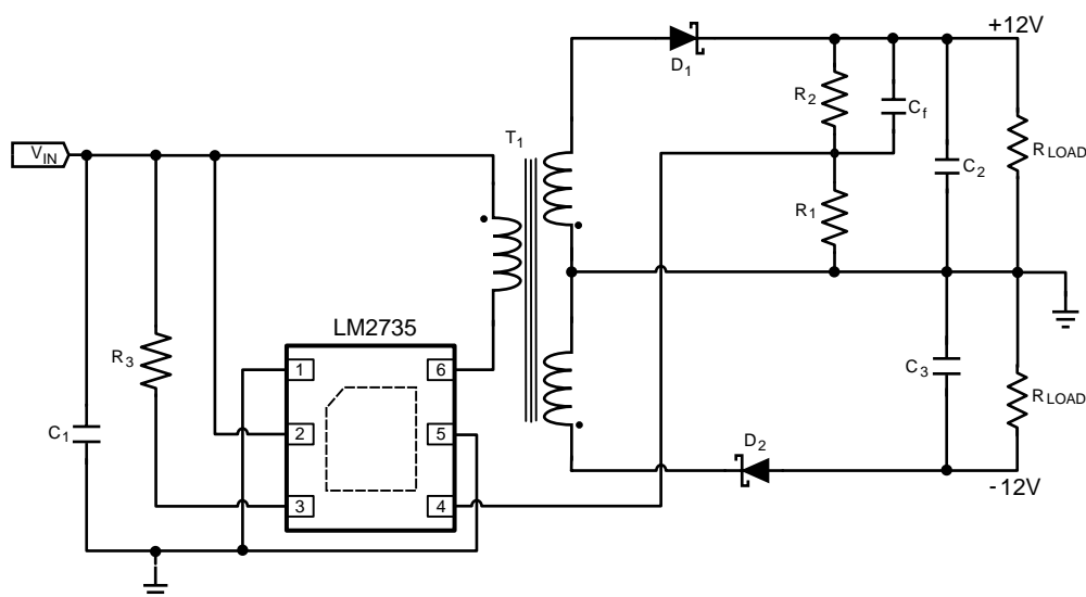
Figure 39. LM2735Y (520kHz): V_{in} = 5V , V_{out} = \pm 12V 150mA
