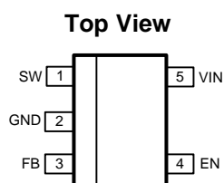
Figure 2. 5-Pin SOT23
