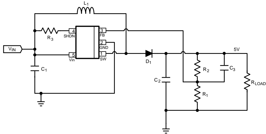
Figure 31. LM2735Y (520kHz): V_{in} = 3V , V_{out} = 5V @ 750mA
