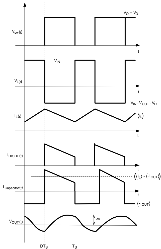
Figure 7. Typical Waveforms
