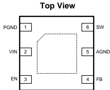
Figure 3. 6-Pin LLP
