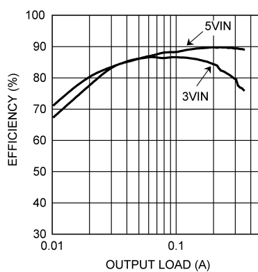
Figure 1. Efficiency vs Load Current V_O = 12V
