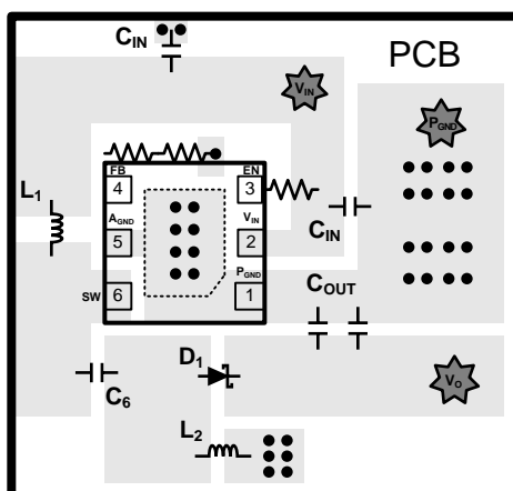
Figure 22. SEPIC PCB Layout
