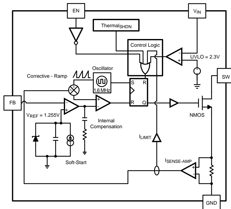
Figure 5. Simplified Block Diagram
