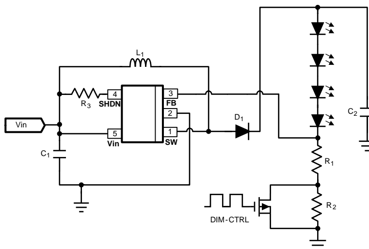
Figure 38. LM2735X (1.6MHz): V_{in} = 2.7V - 5V , V_{out} = 20V @ 50mA
