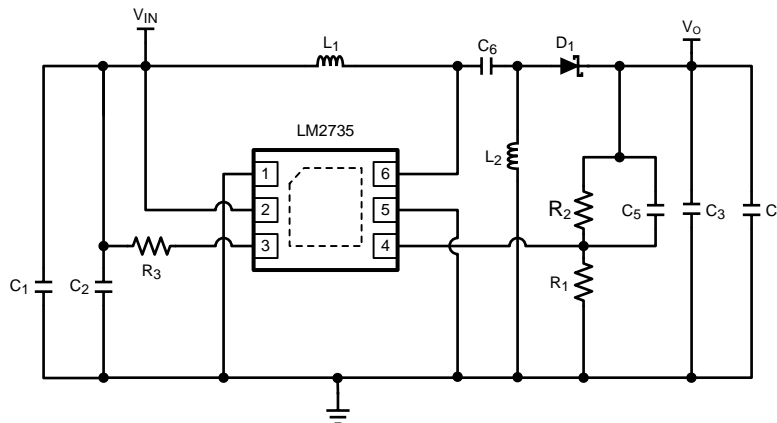
Figure 20. SEPIC CONVERTER Schematic
