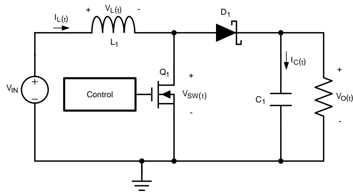
Figure 6. Simplified Schematic
