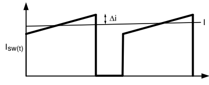
Figure 17. LM2735 Switch Current
