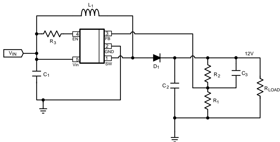
Figure 26. LM2735Y (520kHz): V_{in} = 5V , V_{out} = 12V @ 350mA
