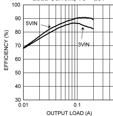
LM2735Y Efficiency vs
