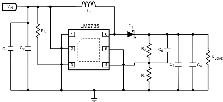
Figure 27. LM2735X (1.6MHz): V in = 3.3V, V out = 12V @ 350mA
