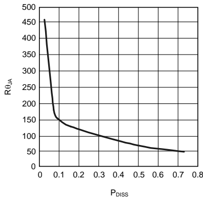
Figure 18. R θJA vs Internal Dissipation for the LLP-6 and eMSOP-8 Package
