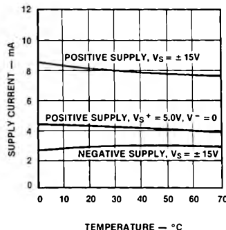
SUPPLY CURRENTS (LM319)
