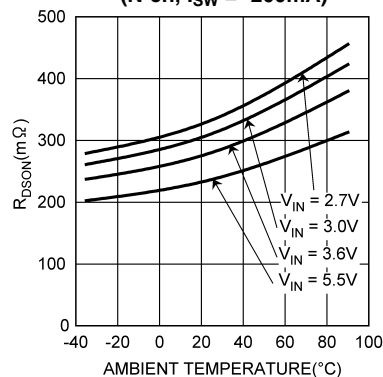
R_{DS(on)} vs Temperature (microSMD) (N-ch, I_{SW} = -200\text{mA} )
