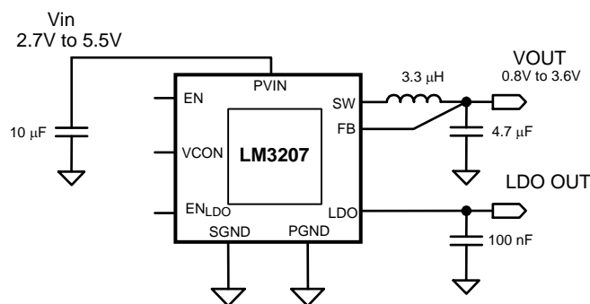
Figure 1. LM3207 Typical Application
