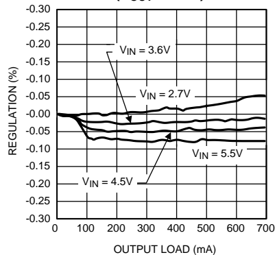
Output Voltage Regulation(%) vs Output Load ( V_{OUT} = 1.5V )
