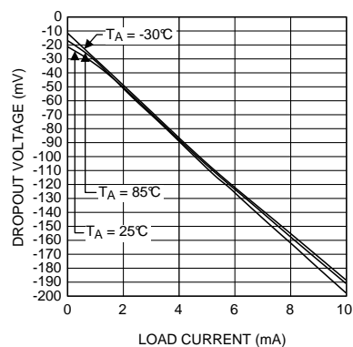
LDO Dropout Voltage vs Load Current ( C_{LDO} = 100\text{nF} ), (1)
