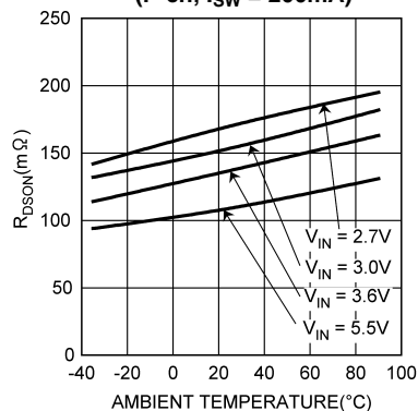
R_{DS(on)} vs Temperature (microSMD) (P-ch, I_{SW} = 200\text{mA} )
