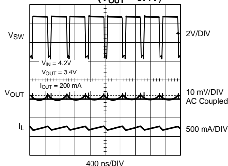
Output Voltage Ripple ( V_{OUT} = 3.4V )
