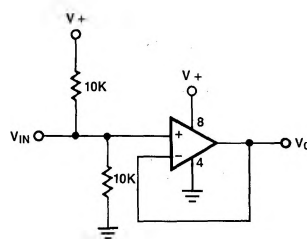
INPUT BIASING VOLTAGE FOLLOWER
