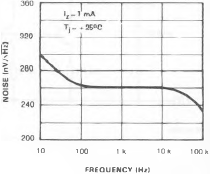
NOISE VOLTAGE
