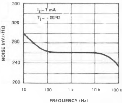
NOISE VOLTAGE
