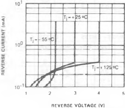
REVERSE CHARACTERISTICS
