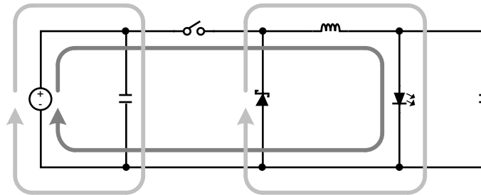
Figure 31. Buck Converter Current Loops
