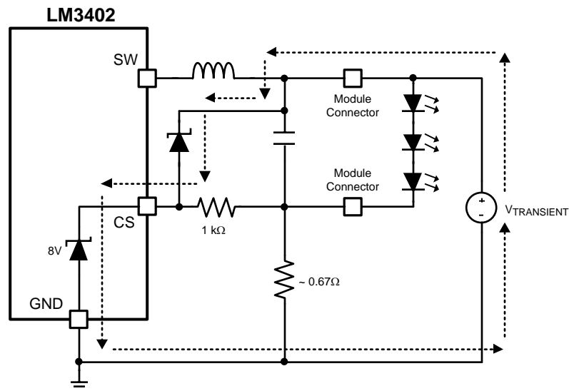
Figure 26. CS Pin with OVP, Transient Path
