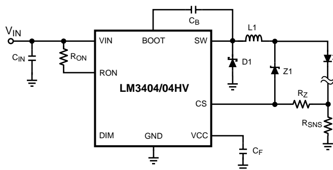
Figure 20. Output Open Circuit Protection
