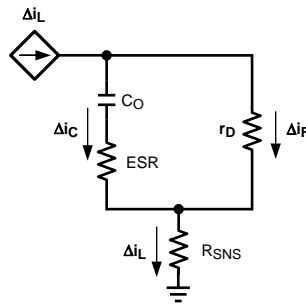
Figure 22. LED and C O Ripple Current
