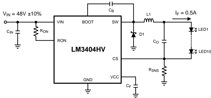
Figure 31. Schematic for Design Example 2
