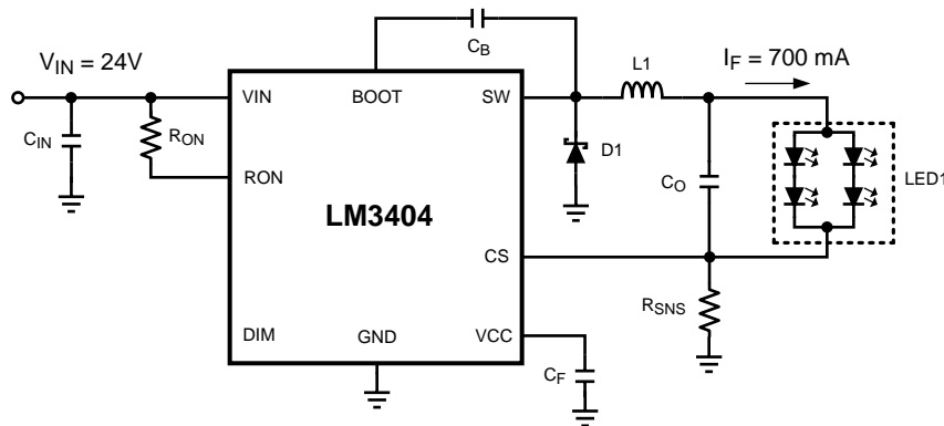
Figure 30. Schematic for Design Example 1
