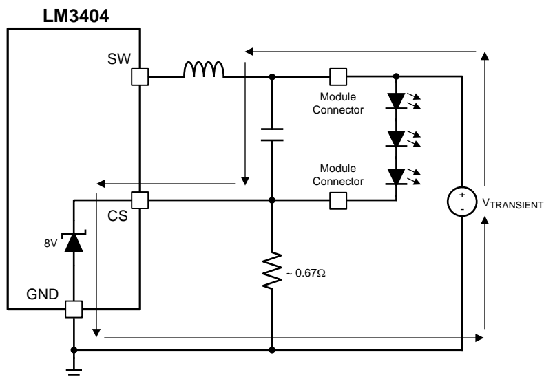
Figure 24. CS Pin, Transient Path
