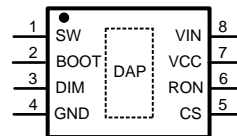
Figure 2. 8-Lead Plastic So PowerPAD-8 Package
