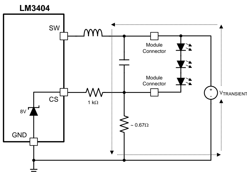
Figure 25. CS Pin, Transient Path with Protection
