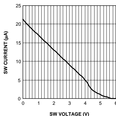
Figure 23. LED Current From SW Pin
