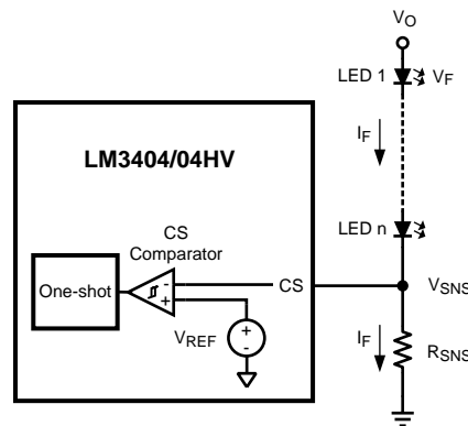
Figure 19. Comparator and One-Shot
