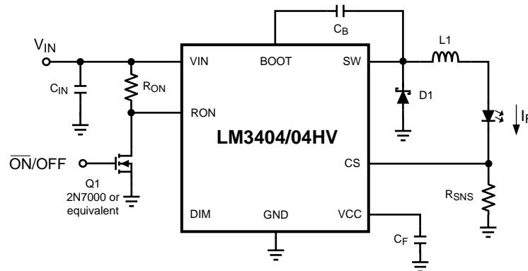
Figure 21. Low Power Shutdown
