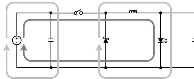
Figure 32. Buck Converter Current Loops
