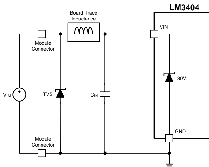
Figure 28. VIN Pin with Typical Input Protection
