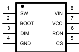
Figure 1. 8-Lead Plastic SOIC-8 Package
