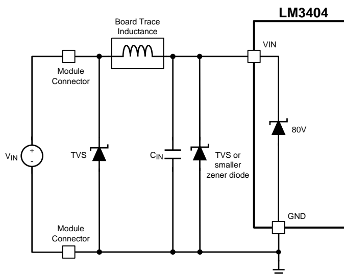
Figure 29. VIN Pin with Additional Input Protection
