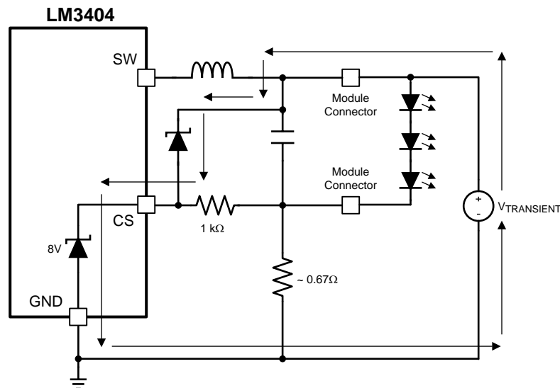
Figure 26. CS Pin with OVP, Transient Path
