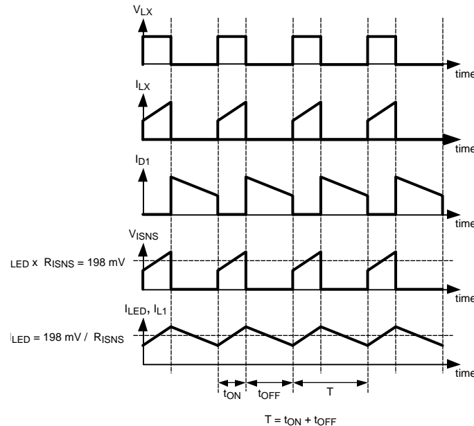
Figure 19. Operating Waveforms of a Floating Buck Converter
