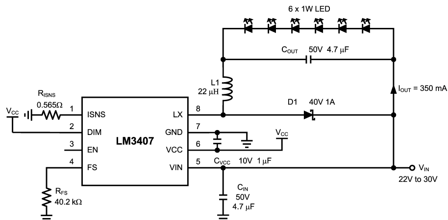
Figure 25. Typical Application Schematic for 6 LEDs
