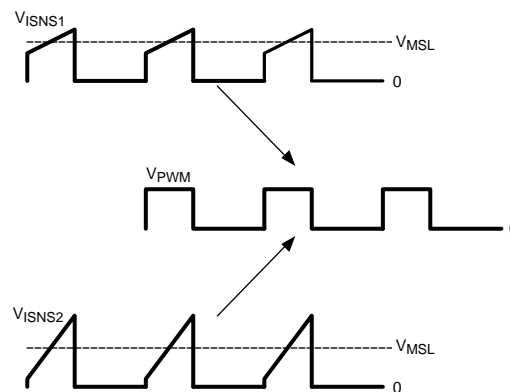
Figure 21. Pulse-Level Transformation
