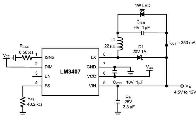
Figure 26. Typical Application Schematic for 1 LED
