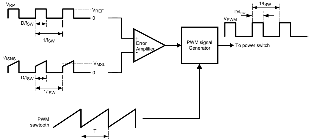
Figure 22. Implementation of the PWM Switching Signal
