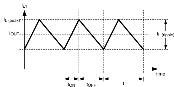
Figure 24. Relationship between I_{OUT} , I_{L(\text{peak})} and I_{L(\text{ripple})}
