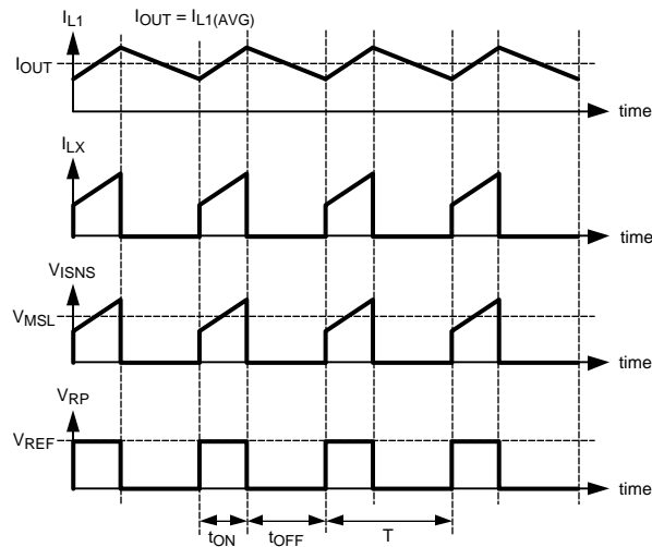
Figure 20. LM3407 Switching Waveforms
