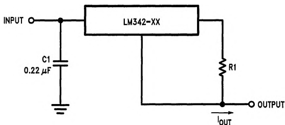
Current Regulator
