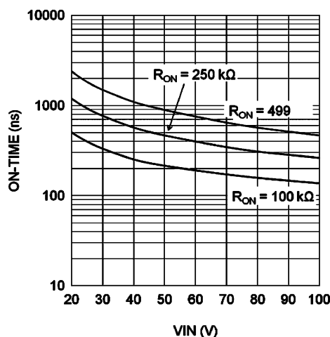
Figure 14. T_{ON} vs V_{IN} and R_{ON}
