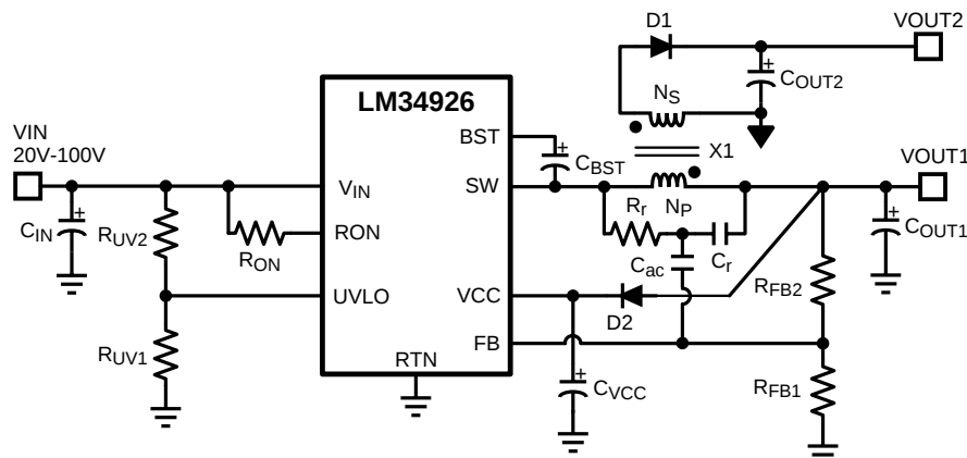
Figure 16. Typical Isolated Application Schematic
