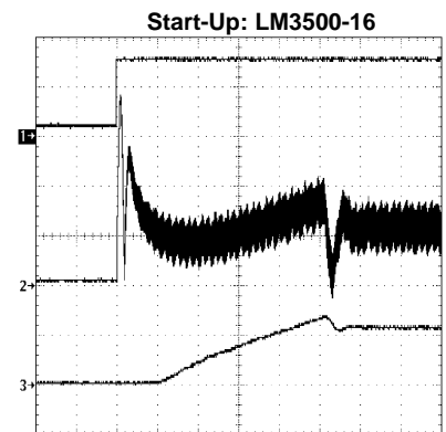
3 LEDs, R_{LED} = 22\Omega , V_{IN} = 3.0V 1) SHDN, 1V/div, DC 2) I_L , 100mA/div, DC 3) I_{LED} , 20mA/div, DC T = 100µs/div
