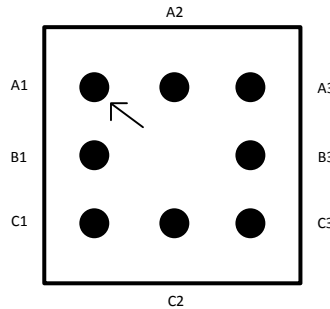
Figure 1. 8-bump DSBGA
