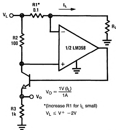
Current Monitor
