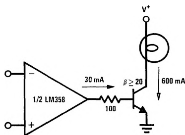
Lamp Driver
