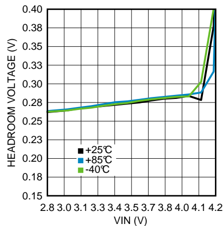
Flash Headroom Voltage vs. V_{IN} V_{LED} = 3.8V , I_{LED} = 1A
