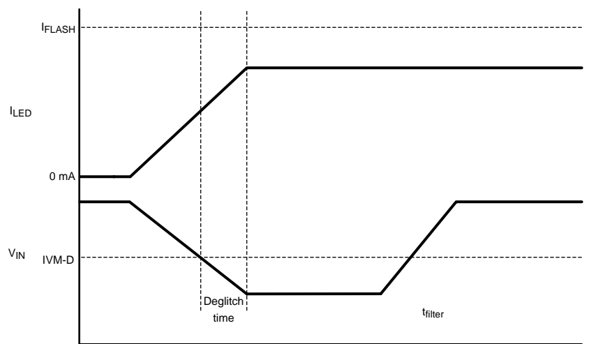
Figure 8. Stop and Hold Mode
