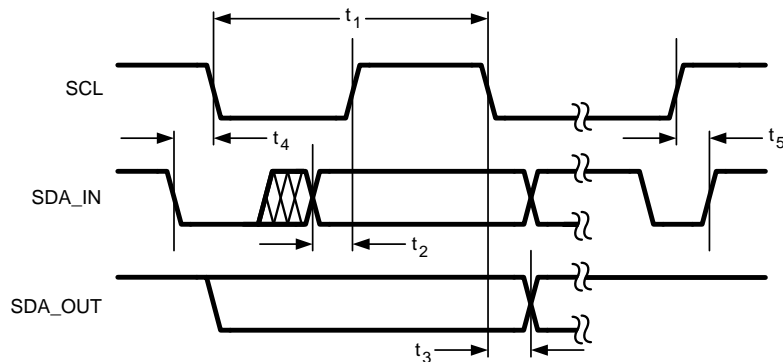
Figure 3. I 2 C-Compatible Interface Specifications
