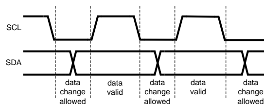
Figure 4. Data Validity Diagram
