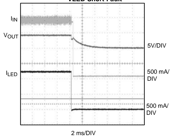
VLED Short Fault
