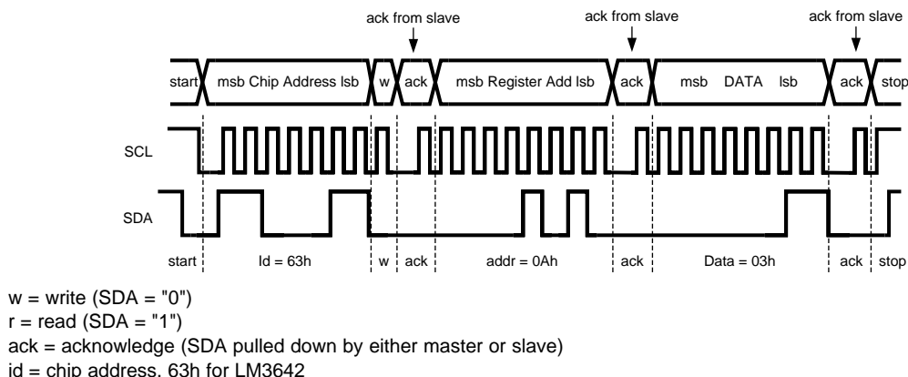
Figure 6. Write Cycle
