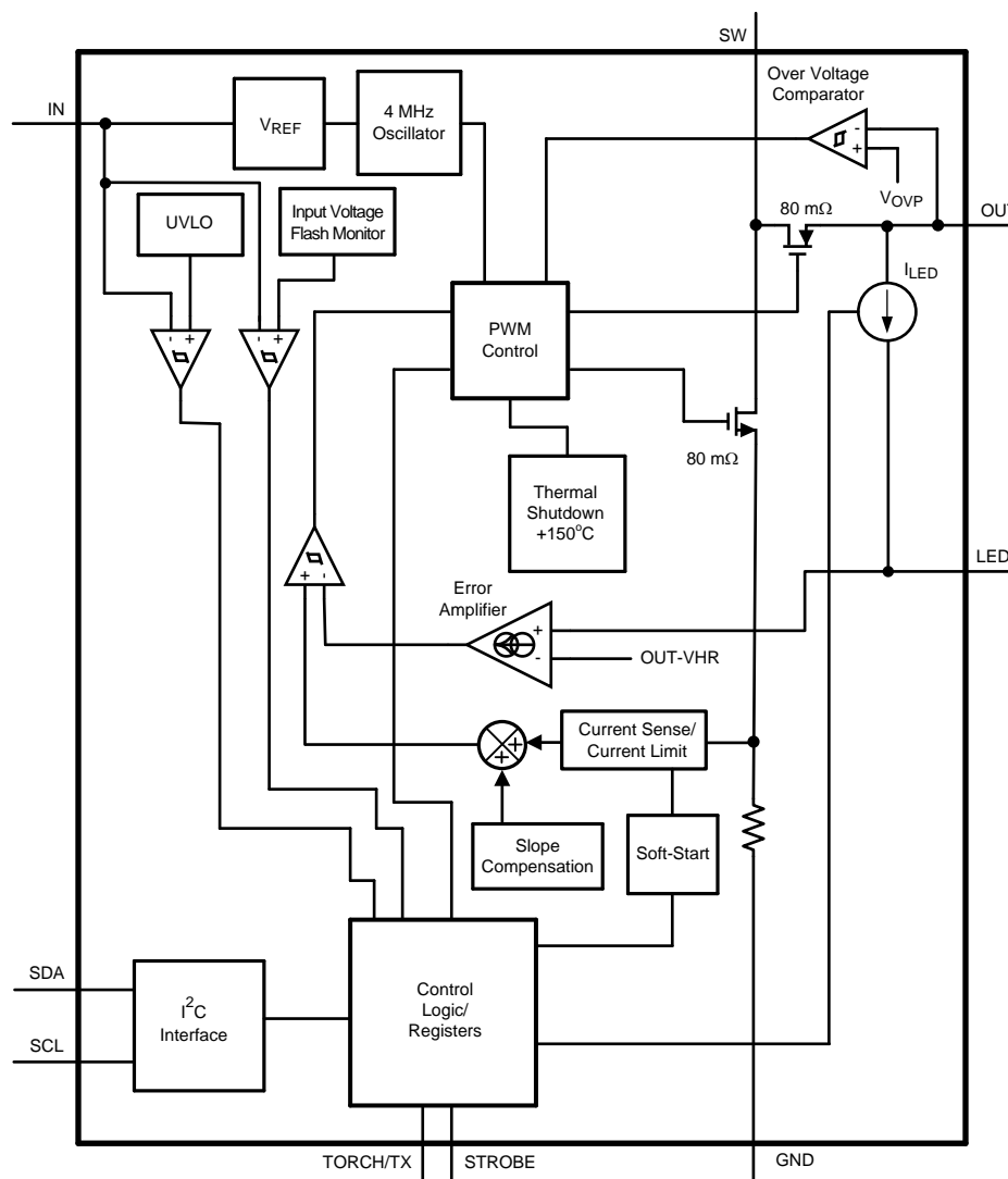
Figure 2. Block Diagram
