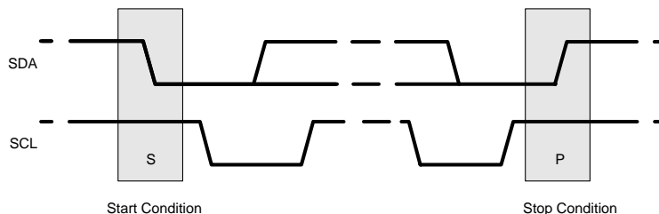
Figure 5. Start and Stop Conditions
