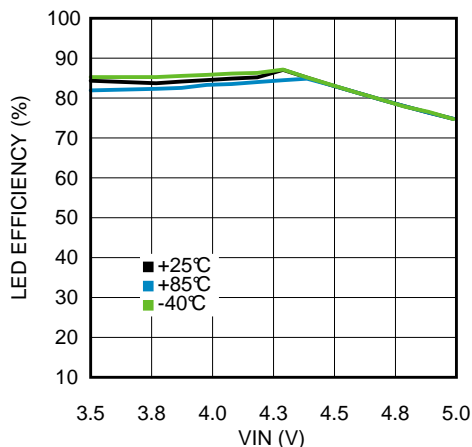
Torch LED Efficiency vs. V_{IN} V_{LED} = 3.7V , I_{LED} = 375mA
