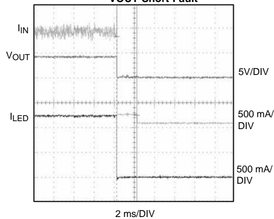
VOUT Short Fault
