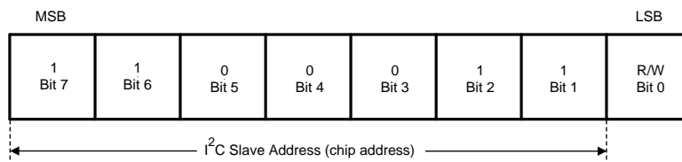
Figure 7. I 2 C-Compatible Device Address
