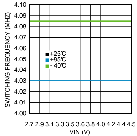
Switching Frequency vs. V_{IN} VLED = 3.8V
