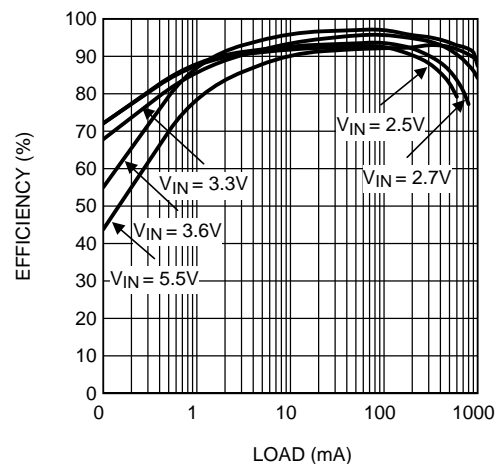
Figure 2. Efficiency at 3.3V Output
