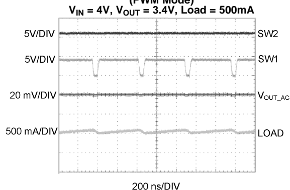
Typical Switching Waveform in Buck Mode (PWM Mode)
