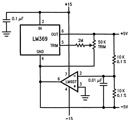
±5V Reference
