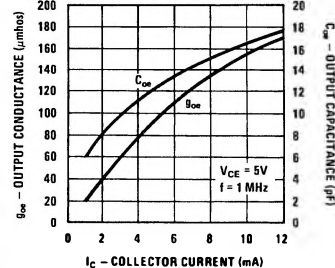
g_{oe} and C_{oe} vs Collector Current
