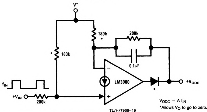
Tachometer
