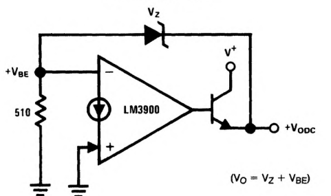
Voltage Regulator
