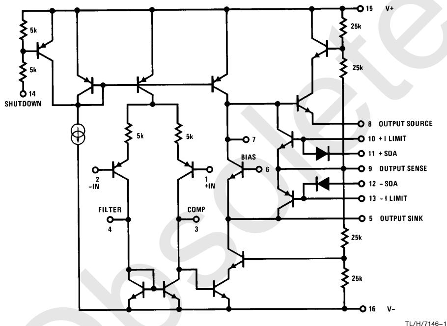
Dual-In-Line Package
