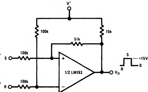
Bi-Stable Multivibrator
