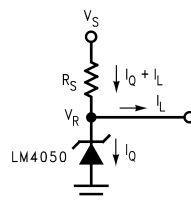
Figure 12. Shunt Regulator
