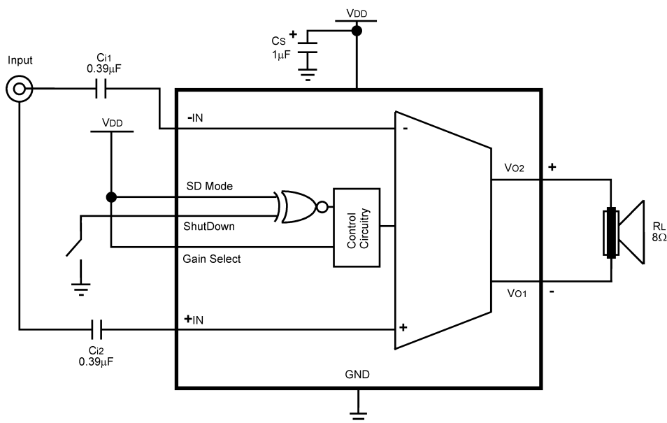
Figure 9. Single-Ended Input, Shutdown High and Gain of 6dB Configuration
