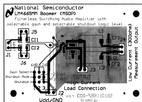
Figure 13. Composite View
