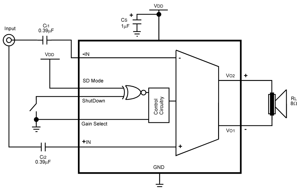
Figure 10. Single-Ended Input, Shutdown High and Gain of 12dB Configuration
