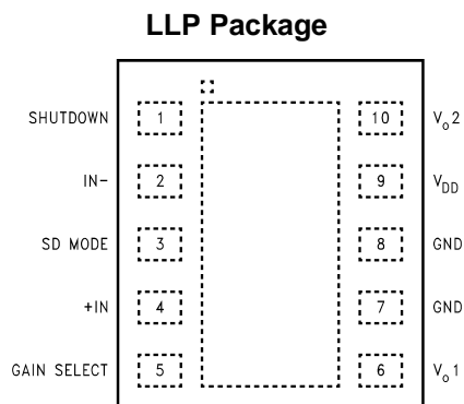
Figure 4. Top View Order Number LM4665LD See NS Package Number LDA10B
