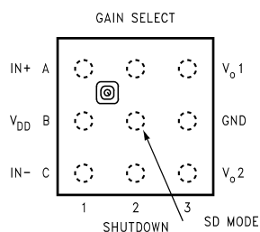
Figure 3. Top View Order Number LM4665ITL, LM4665ITLX See NS Package Number TLA09AAA
