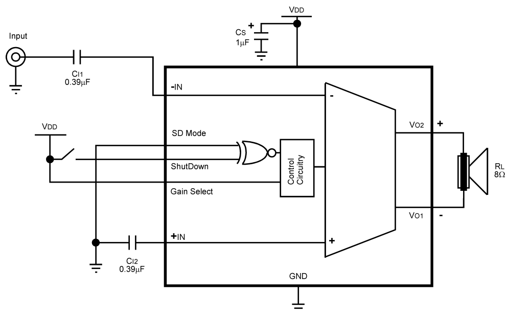
Figure 11. Single-Ended Input, Shutdown Low and Gain of 6dB Configuration
