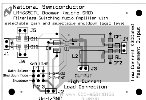
Figure 22. Silk Screen
