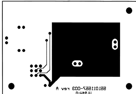
Figure 16. Bottom Layer
