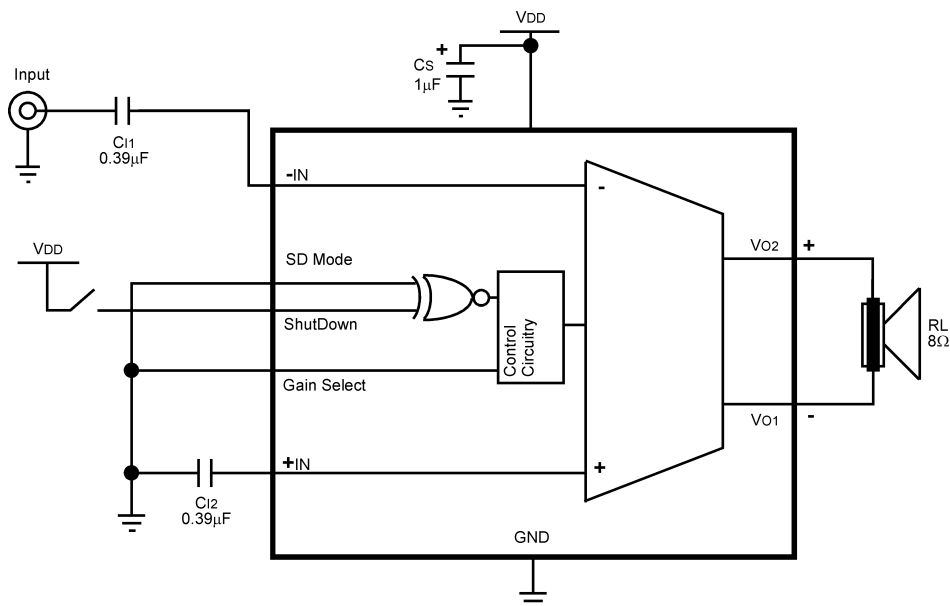
Figure 12. Single-Ended Input, Shutdown Low and Gain of 12dB Configuration
