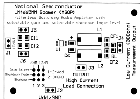
Figure 15. Top Layer
