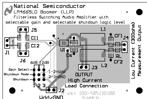
Figure 18. Silk Screen
