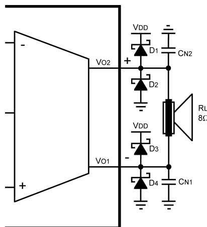
Figure 8. Increased Supply Voltage Operating Range for the micro SMD package
