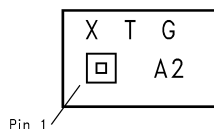
Figure 6. Top View X - Date Code T- Die Traceability G - Boomer Family A2 - LM4665ITL
