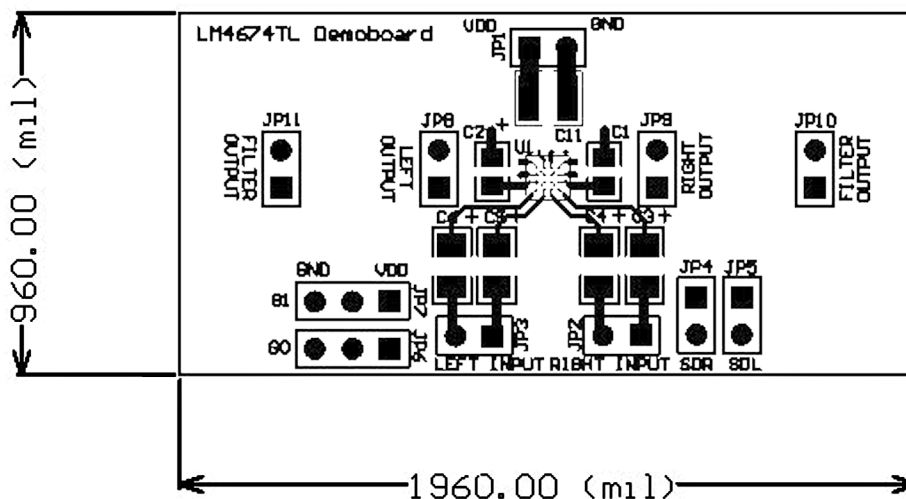
LM4674TL DEMONSTRATION BOARD LAYOUT
