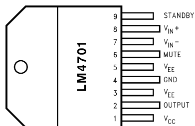
Plastic Package Top View
