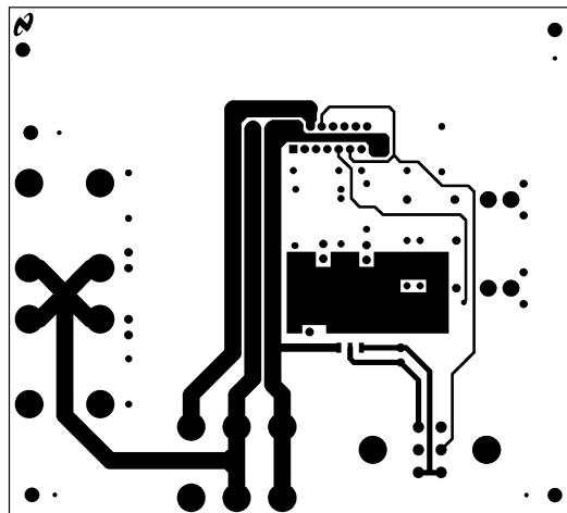
Figure 11. Top Layer
