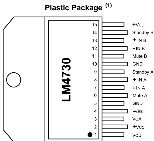
Figure 1. Top View Non-Isolated Package Order Number LM4730TA See NS Package Number TA15A
