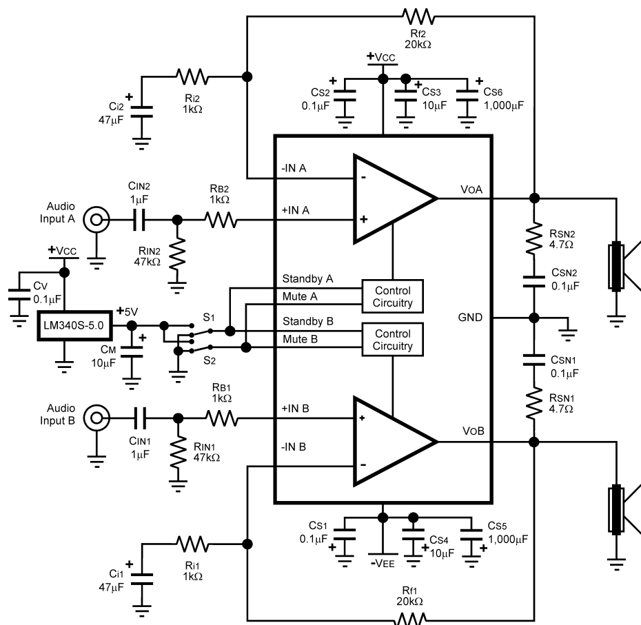
Figure 8. Reference PCB Schematic
