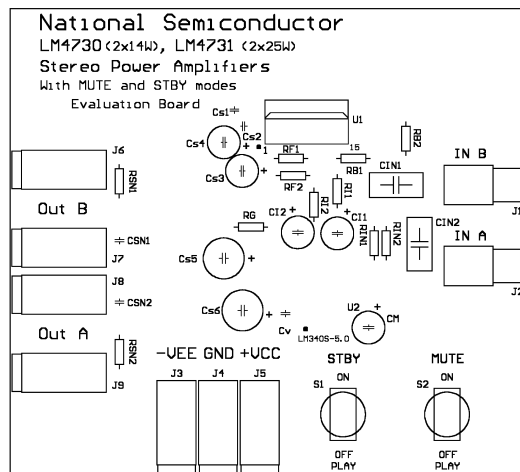
Figure 10. Silk Screen
