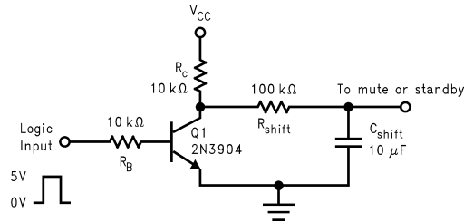
Figure 7. Level Shift Circuit
