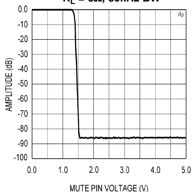
Mute Attenuation vs Mute Pin Voltage \pm 17\text{V} , P_O = 1\text{W} , R_L = 8\Omega , 80kHz BW
