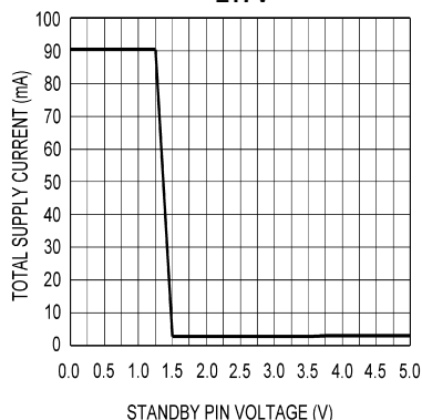
Supply Current vs Standby Pin Voltage \pm 17\text{V}
