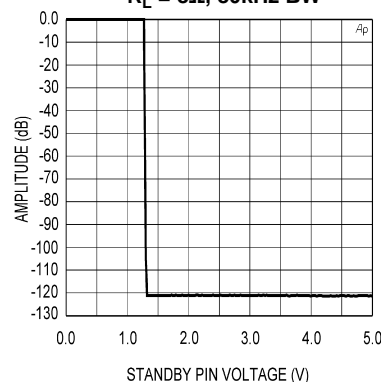
Standby Attenuation vs Standby Pin Voltage \pm 17\text{V} , P_O = 1\text{W} , R_L = 8\Omega , 80kHz BW
