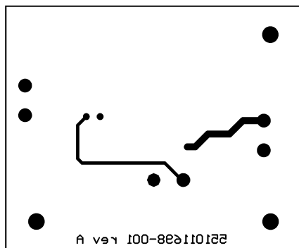
Figure 9. Bottom Layer
