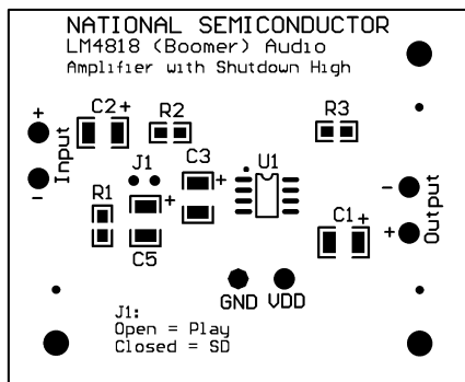
Figure 7. Silk Screen
