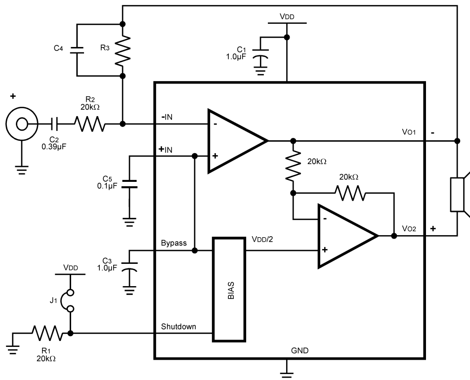
Figure 4. HIGHER GAIN AUDIO AMPLIFIER
