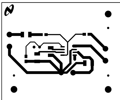
Figure 8. Top Layer
