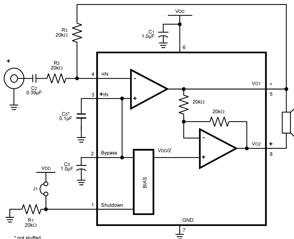
Figure 5. REFERENCE DESIGN BOARD and PCB LAYOUT GUIDELINES
