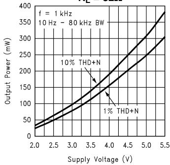
Output Power vs Supply Voltage RL = 32Ω
