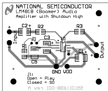
Figure 6. Composite View
