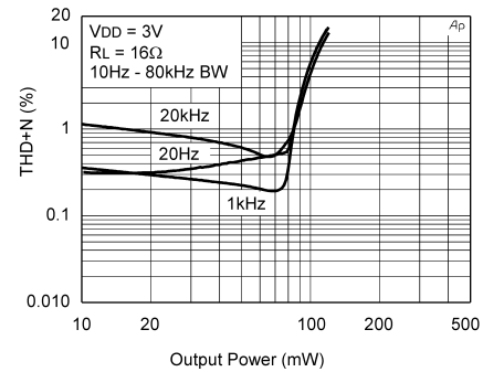
THD+N vs Output Power
