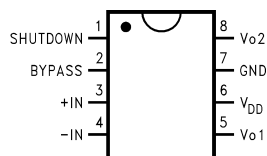
Figure 2. Top View Order Number LM4818M See NS Package Number M08A
