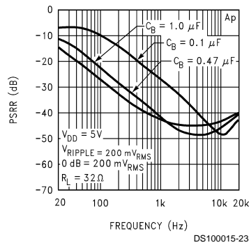
Power Supply Rejection Ratio Line Out/HP Amplifiers
