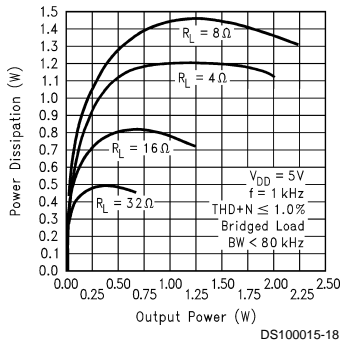
Power Dissipation vs Output Power Bridged Power Amp
