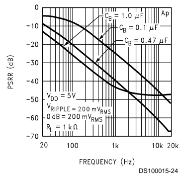
Power Supply Rejection Ratio Mic Preamp
