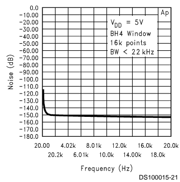
Noise Floor Mic Preamp
