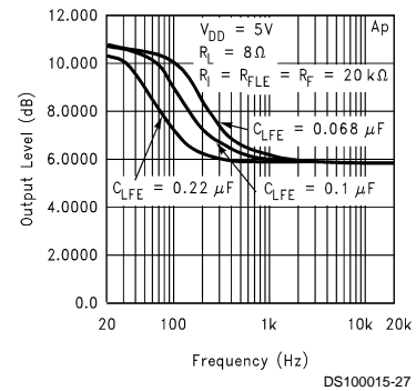
Low Frequency Enhancement Characteristics Bridged Power Amp
