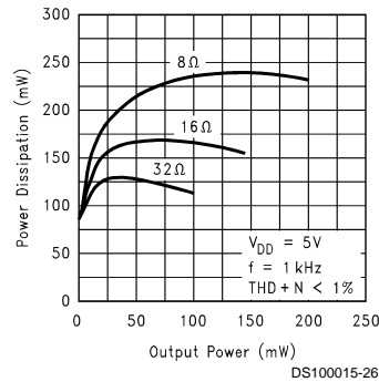
Power Dissipation vs Output Power Line Out/HP Amplifiers
