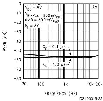
Power Supply Rejection Ratio Bridged Power Amp
