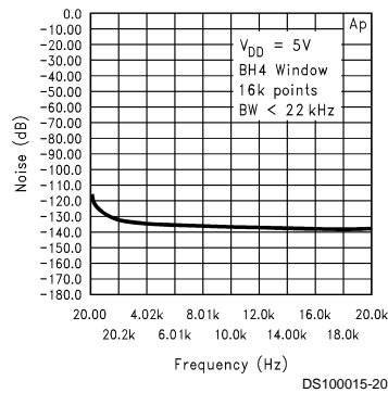
Noise Floor Line Out/HP Amp
