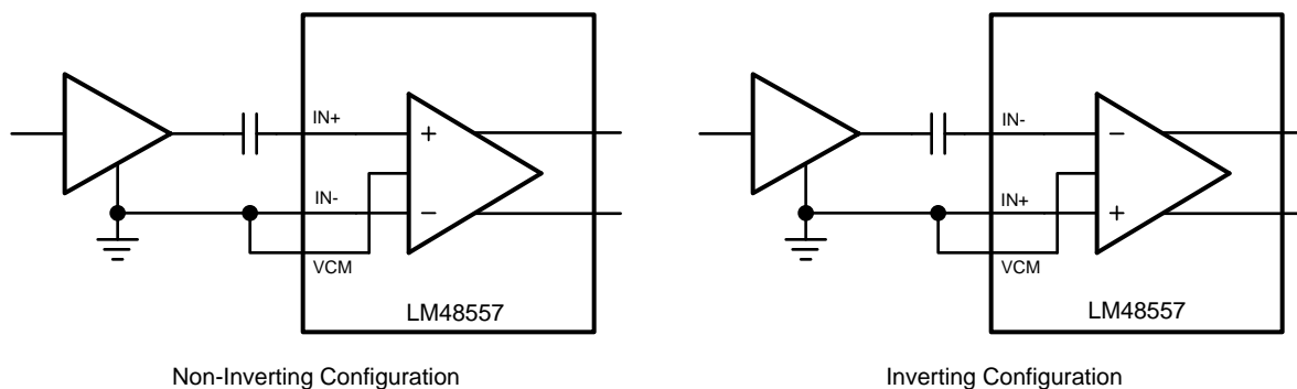
Figure 13. Single-Ended Input Configuration with a Ground-Referenced Source
