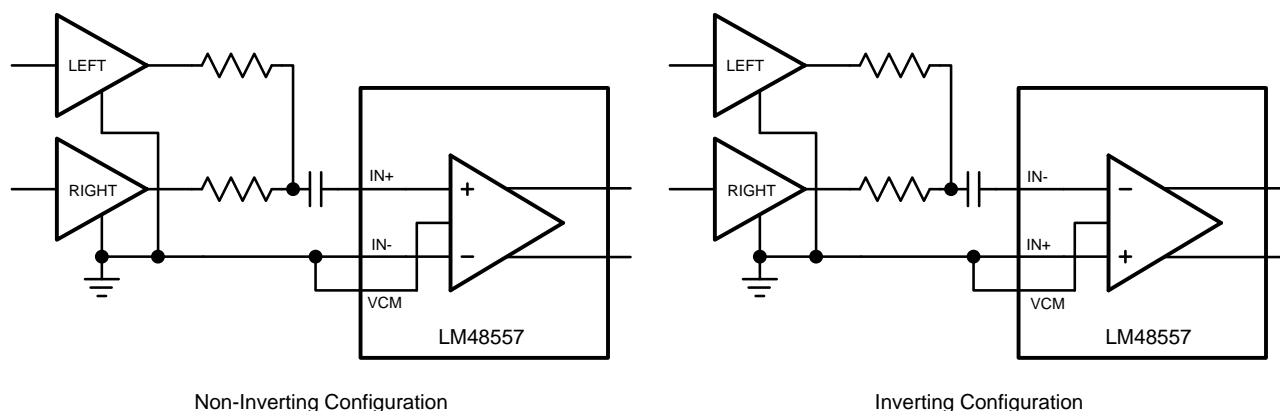
Figure 14. Single-Ended Stereo-to-Mono BTL Conversion
