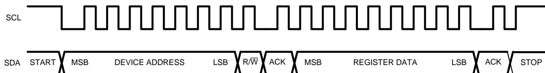
Figure 10. Example Write Sequence
