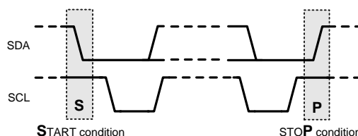
Figure 9. Start and Stop Diagram
