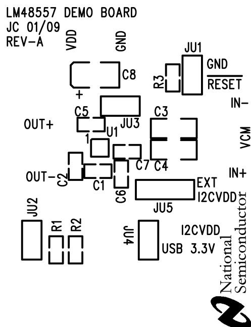
Figure 15. Silk Screen
