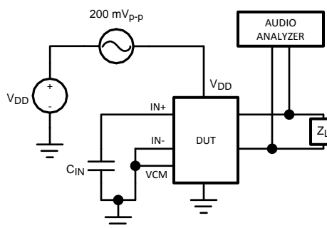
Figure 6. PSRR Test Circuit
