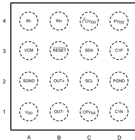
Figure 2. TL Package - Top View
