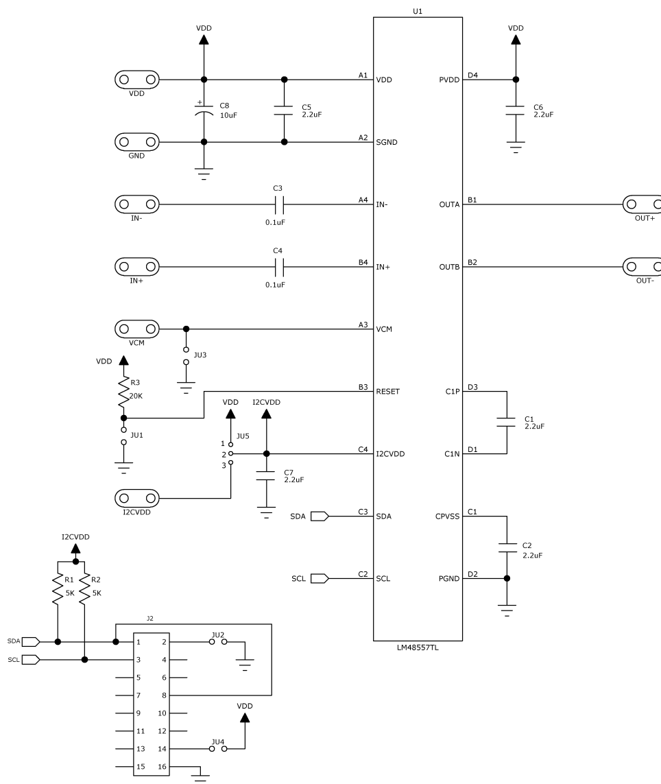
Figure 21. LM48557 Demo Board Schematic
