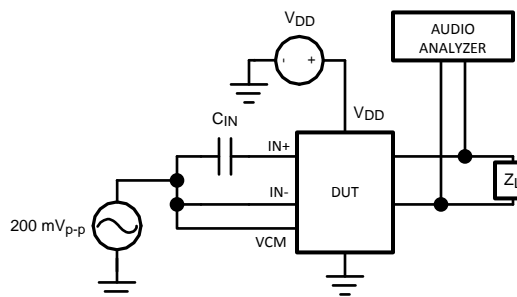
Figure 7. CMRR Test Circuit
