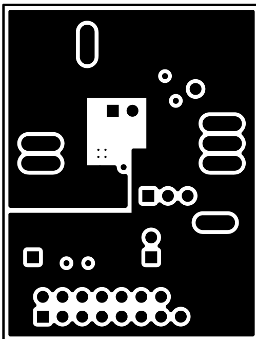
Figure 17. Layer 2
