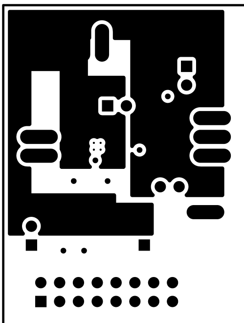
Figure 18. Layer 3
