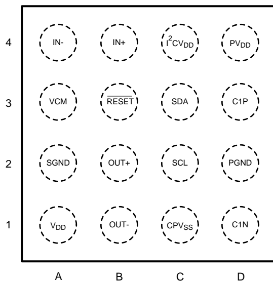
Figure 4. UR Package - Top View
