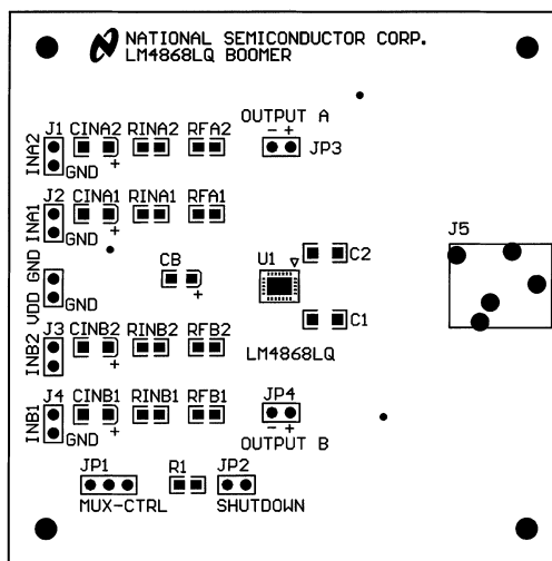
Figure 11. Recommended LQ PC Board Layout: Component-Side Silkscreen
