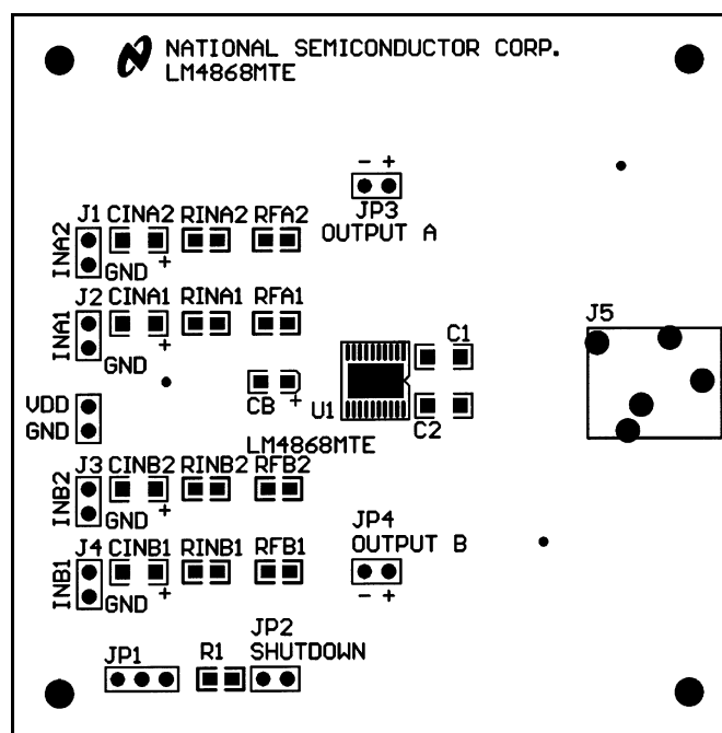
Figure 16. Recommended MTE PC Board Layout: Component-Side Silkscreen
