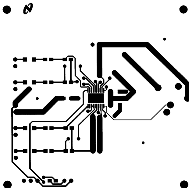
Figure 17. Recommended MTE PC Board Layout: Component-Side Layout
