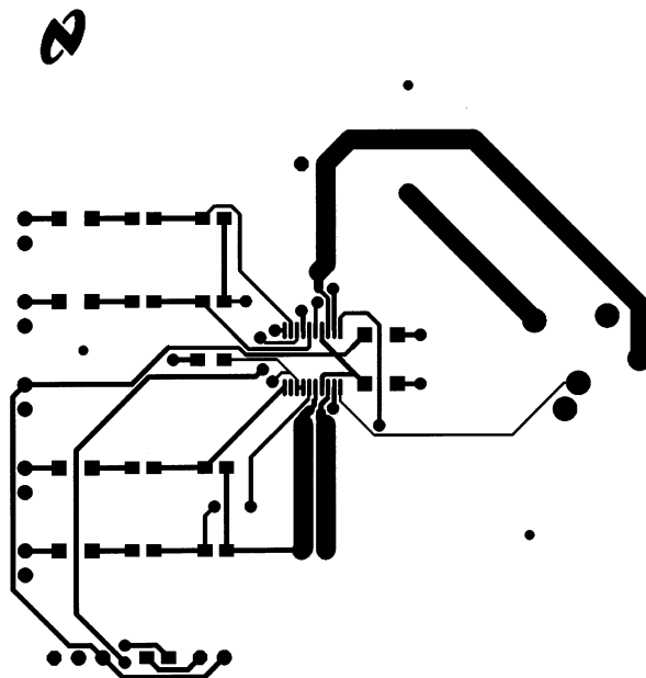
Figure 22. Recommended MT PC Board Layout: Component-Side Layout
