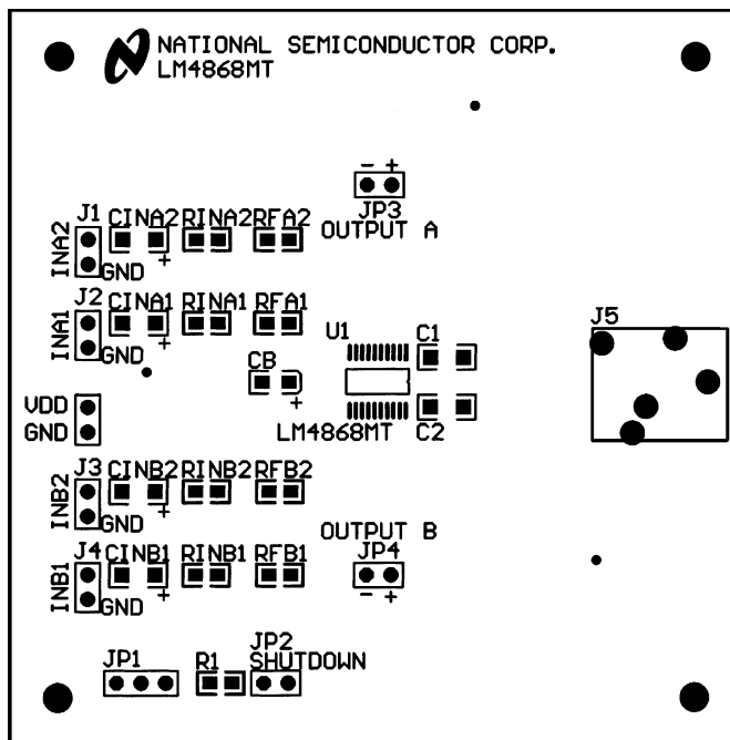
Figure 21. Recommended MT PC Board Layout: Component-Side Silkscreen
