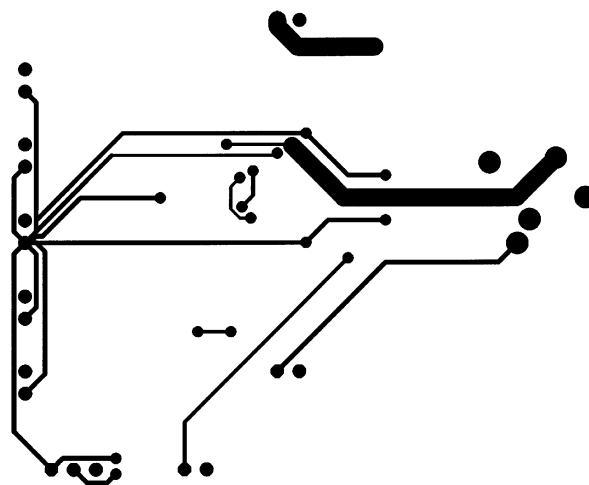
Figure 23. Recommended MT PC Board Layout: Bottom-Side Layout
