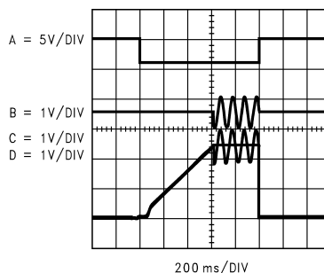
Figure 5. Single-ended output signal (Trace B) is devoid of transients. The SHUTDOWN pin is driven by a shutdown signal (Trace A). The inverting output (Trace C) and the V_{\text{BYPASS}} output (Trace D) are applied across a 32 \Omega BTL load.
