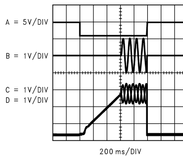
Figure 4. Differential output signal (Trace B) is devoid of transients. The SHUTDOWN pin is driven by a shutdown signal (Trace A). The inverting output (Trace C) and the non-inverting output (Trace D) are applied across an 8\Omega BTL load.
