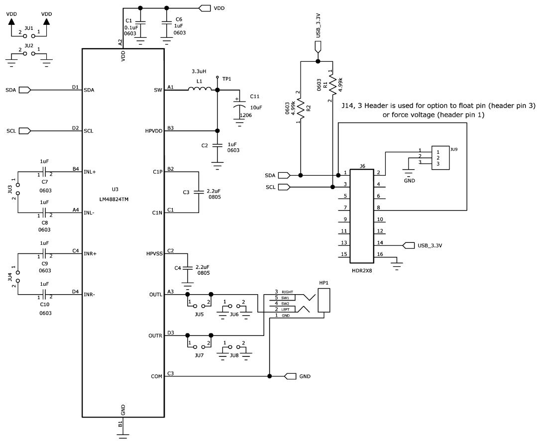
Figure 12. LM48824 Demoboard Schematic
