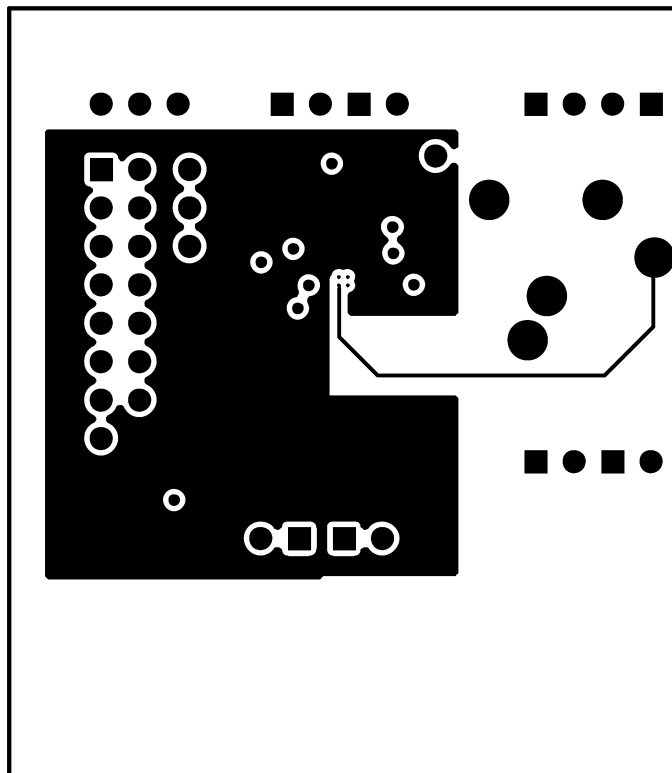
Figure 15. Layer 2 (GND)
