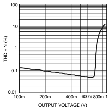
THD+N vs Output Voltage V_{DD} = 3.6V , R_L = 16\Omega , f = 1kHz
