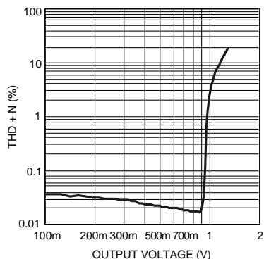
THD+N vs Output Voltage V_{DD} = 3.6V , R_L = 47\Omega , f = 1kHz Low THD Mode
