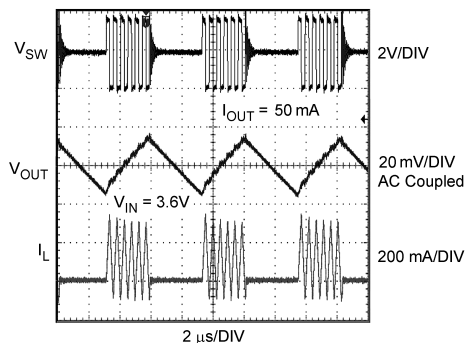
Figure 9. PFM Operation
