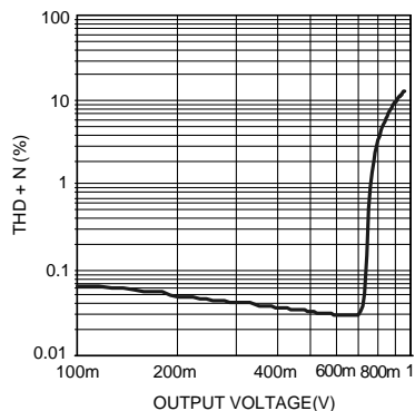
THD+N vs Output Voltage V_{DD} = 3.6V , R_L = 32\Omega , f = 1kHz Low THD Mode
