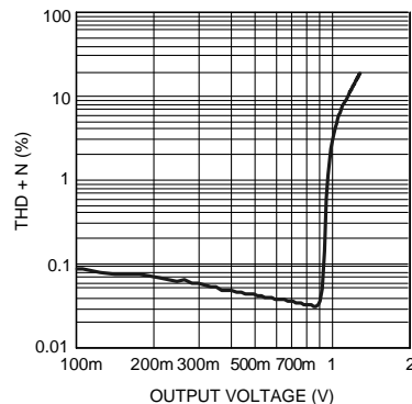
THD+N vs Output Voltage V_{DD} = 3.6V , R_L = 32\Omega , f = 1kHz
