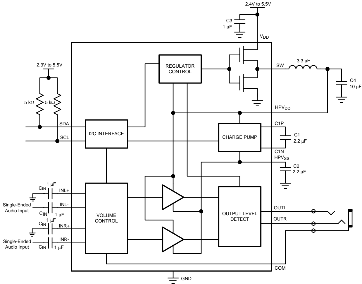
Figure 11. Single-Ended Input Configuration
