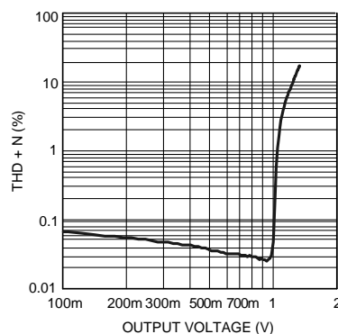
THD+N vs Output Voltage V_{DD} = 3.6V , R_L = 47\Omega , f = 1kHz
