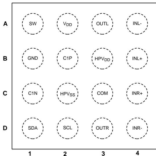
Figure 2. Top View Order Number LM48824TM See NS Package Number TMD16DDA
