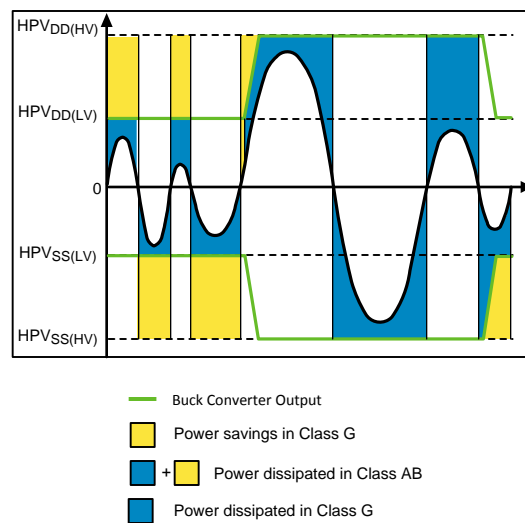
Figure 8. Class G Operation
