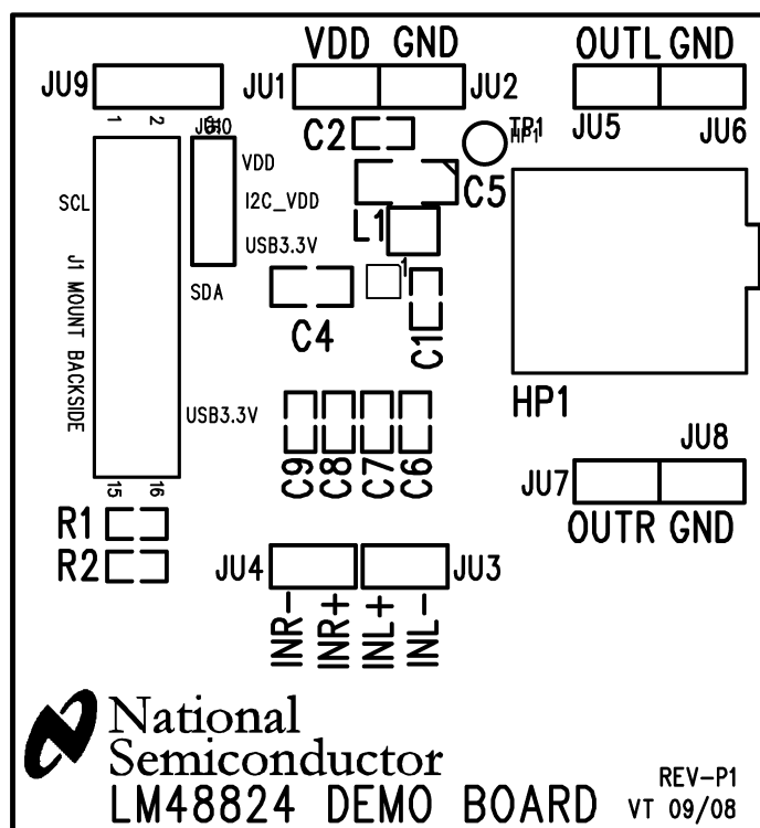
Figure 13. Top Silkscreen
