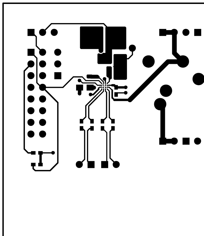
Figure 14. Top Layer
