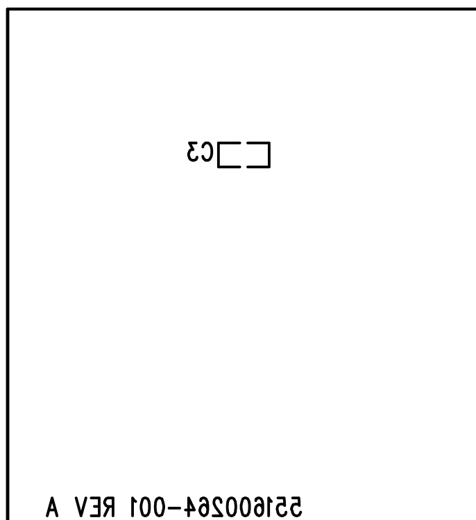
Figure 18. Bottom Silkscreen
