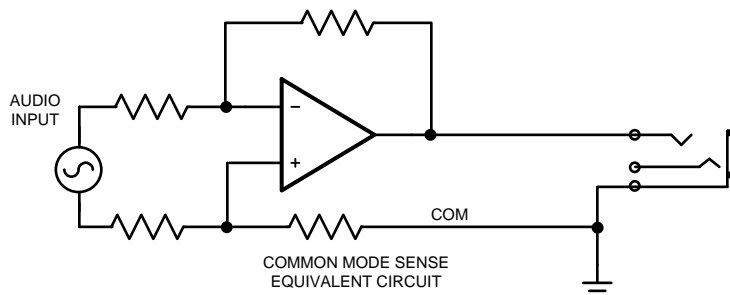
Figure 10. COM Connection
