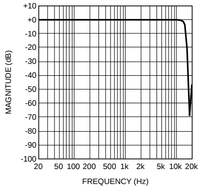
MONO ADC Frequency Response f_s = 32kHz , 36dB MIC
