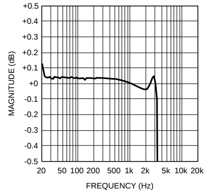
MONO ADC Frequency Response Zoom f_s = 8kHz, 36dB MIC
