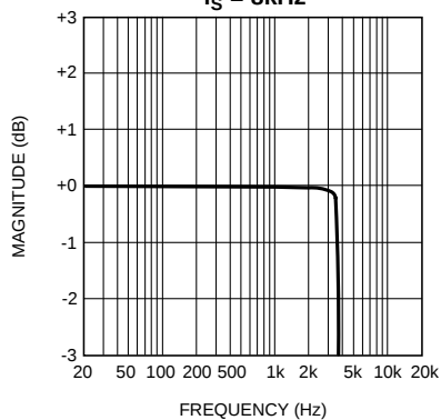
Stereo DAC Frequency Response
