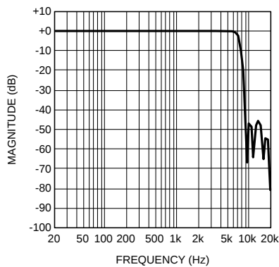
MONO ADC Frequency Response f_s = 16kHz, 6dB MIC
