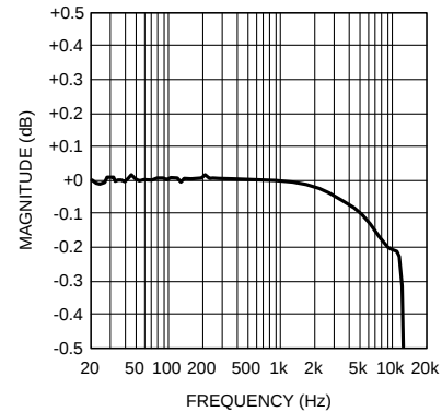
MONO ADC Frequency Response Zoom f_s = 32kHz , 36dB MIC
