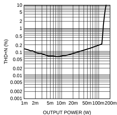
Headphone THD+N vs Output Power AV_{DD} = 5V , SE, 12dB DAC f_{OUT} = 1kHz , 32 \Omega
