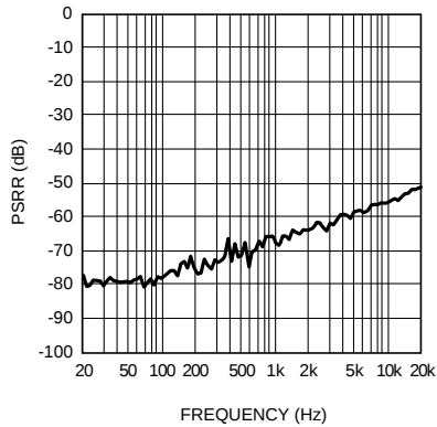
AUXOUT PSRR vs Frequency AV_{DD} = 3.3V , 0dB AUX (AUX inputs terminated)
