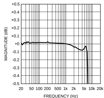
MONO ADC Frequency Response Zoom f_s = 16kHz, 36dB MIC
