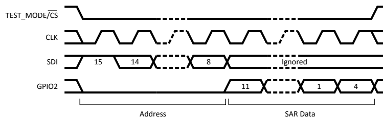
Figure 22. SPI SAR Read Transaction (GPIO2 set to SPI_SDO)
