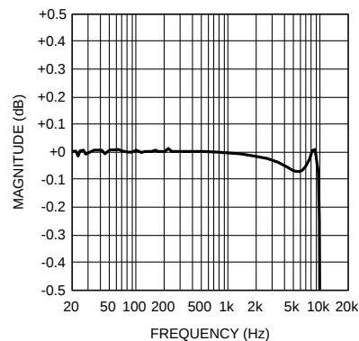
MONO ADC Frequency Response Zoom f_s = 24kHz , 36dB MIC
