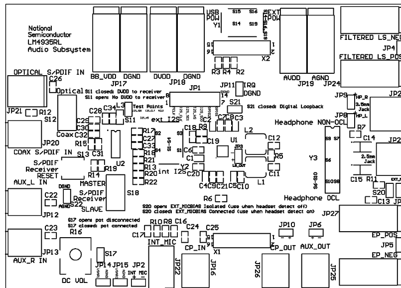
Figure 23. Top Silkscreen
