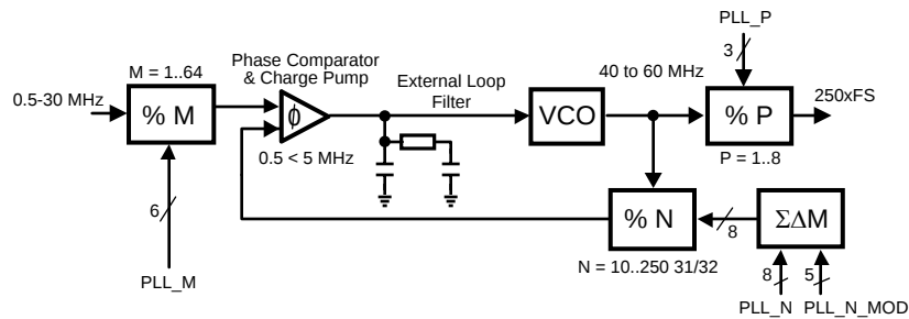
Figure 14. PLL Overview
