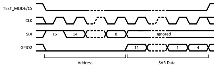
Figure 11. SPI Read Transaction
