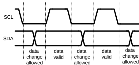
Figure 5. I 2 C Signals: Data Validity
