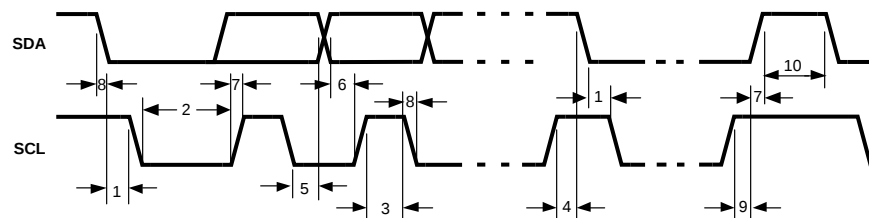
Figure 9. I 2 C Timing Diagram
