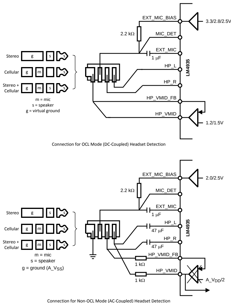
Figure 17. Connection of Headset Jack to LM4935 Depends on the Mode of the Headphone Amplifier.
