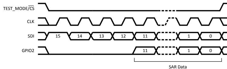
Figure 21. SPI SAR Read Transaction (GPIO2 set to SAR_SDO)
