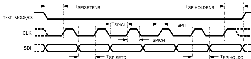
Figure 12. SPI Timing - Three Wire Mode Write Bus Timing
