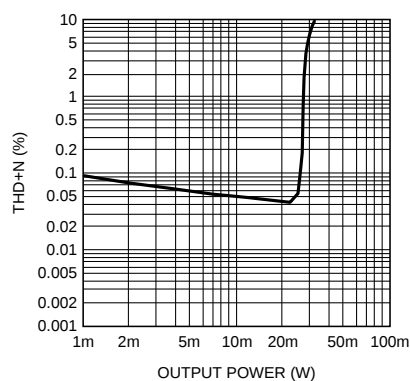
Headphone THD+N vs Output Power AV_{DD} = 3.3V , OCL 1.2V, 0dB AUX f_{OUT} = 1kHz , 16 \Omega
