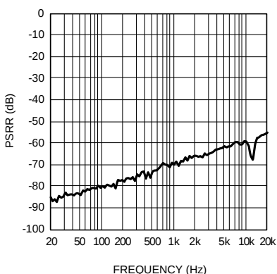
MONO ADC PSRR vs Frequency AV_{DD} = 3.3V , 6dB MIC
