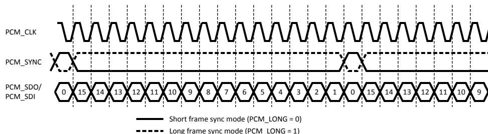
Figure 19. PCM Serial Data Format (16 bit Slave Example)
