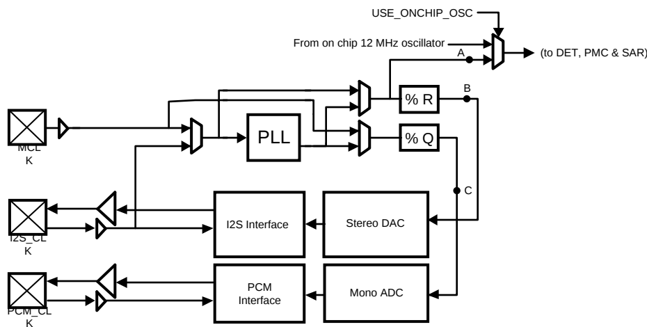
Figure 13. LM4935 Clock Network
