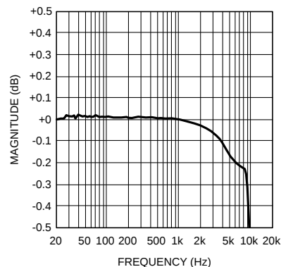
MONO ADC Frequency Response Zoom f_s = 32kHz , 6dB MIC
