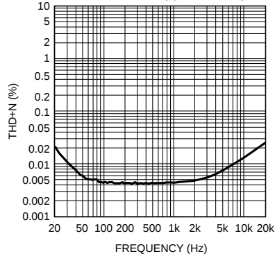
AUXOUT THD+N vs Frequency AV_{DD} = 5V , 0dB, V_{OUT} = 1V_{RMS} , 5k \Omega
