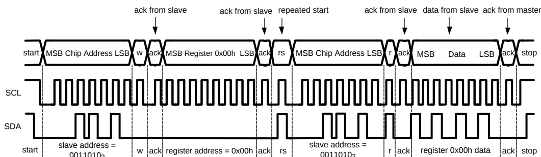
Figure 8. Example I 2 C Read Cycle
