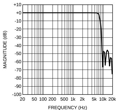
MONO ADC Frequency Response f_s = 16kHz, 36dB MIC
