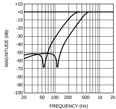
MONO ADC HPF Frequency Response f_s = 16kHz , 36dB MIC (from left to right: HPF_MODE '00', '10', '01')
