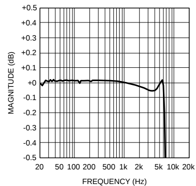
MONO ADC Frequency Response Zoom f_s = 16kHz, 6dB MIC
