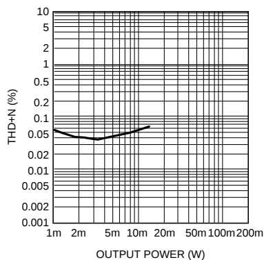
Headphone THD+N vs Output Power AV_{DD} = 5V , SE, 0dB DAC f_{OUT} = 1kHz , 32\Omega
