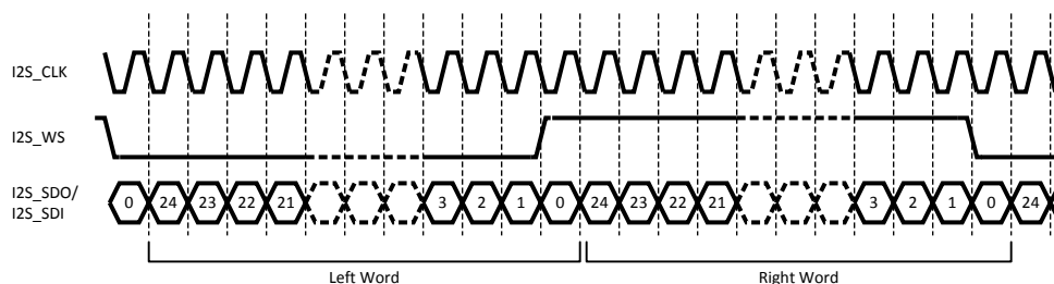
Figure 18. I 2 S Serial Data Format (Default Mode)
