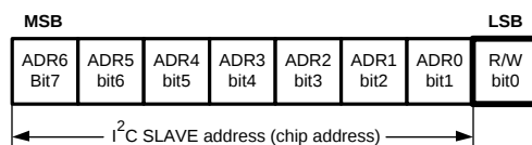
Figure 6. I 2 C Chip Address
