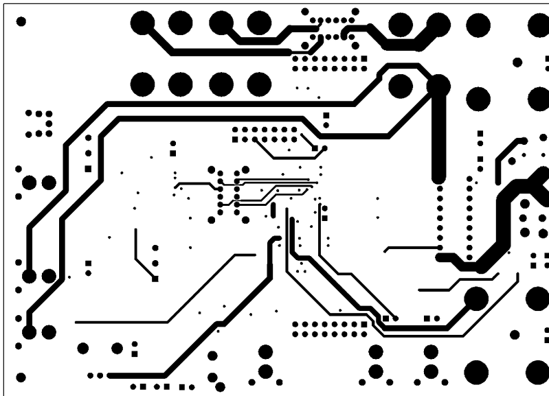
Figure 26. Mid Layer 2
