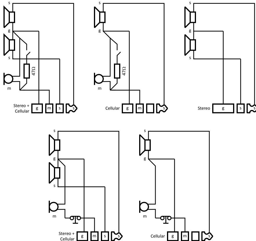
Figure 16. Headset Configurations Supported by the LM4935
