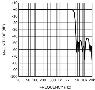
MONO ADC Frequency Response f_s = 8kHz, 36dB MIC
