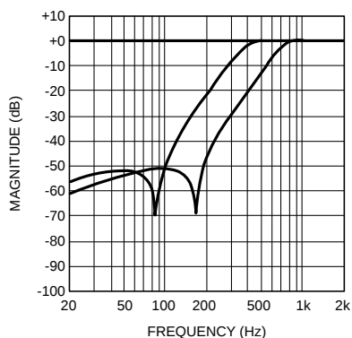
MONO ADC HPF Frequency Response f_S = 24kHz , 36dB MIC (from left to right: HPF_MODE '00', '10', '01')
