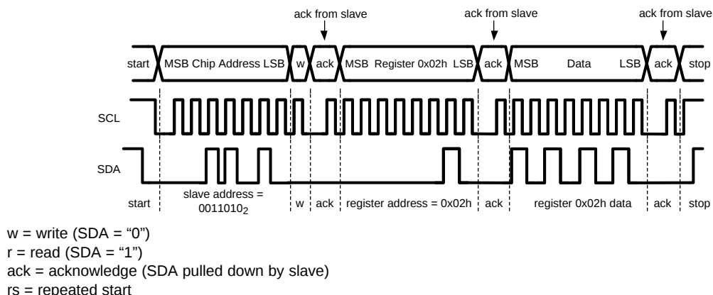
Figure 7. Example I 2 C Write Cycle
