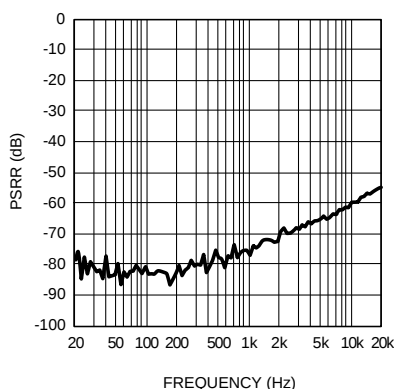
MONO ADC PSRR vs Frequency AV_{DD} = 5V , 6dB MIC
