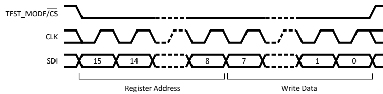
Figure 10. SPI Write Transaction
