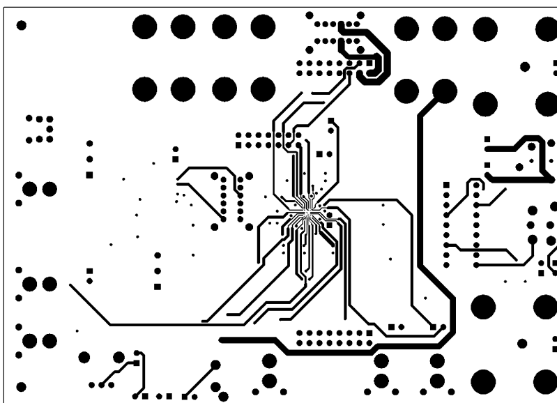
Figure 25. Mid Layer 1
