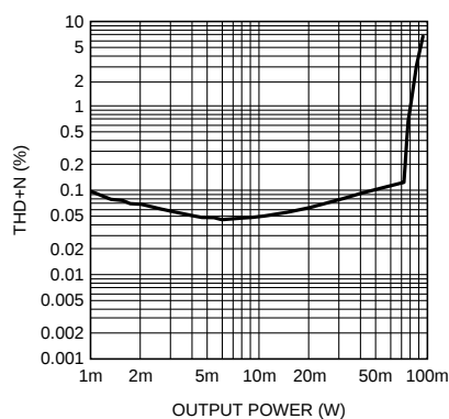
Headphone THD+N vs Output Power AV_{DD} = 5V , SE, 12dB DAC f_{OUT} = 1kHz , 32 \Omega
