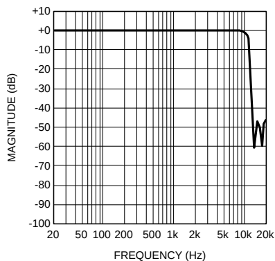
MONO ADC Frequency Response f_s = 24kHz , 36dB MIC
