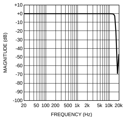
MONO ADC Frequency Response f_s = 32kHz , 6dB MIC
