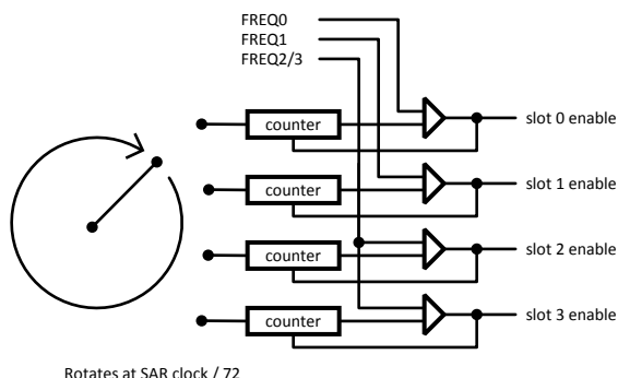
Figure 20. Internal SAR Control Signals to SAR Module
