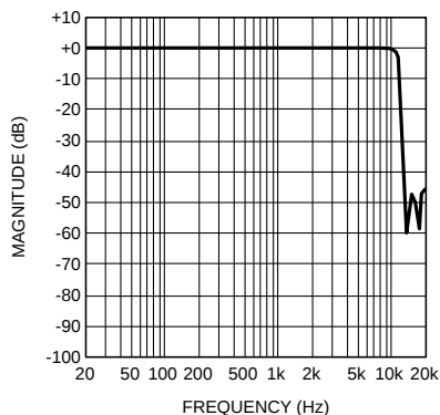
MONO ADC Frequency Response f_s = 24kHz , 6dB MIC
