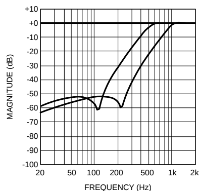
MONO ADC HPF Frequency Response f_S = 32kHz , 36dB MIC (from left to right: HPF_MODE '00', '10', '01')
