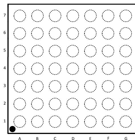
Figure 3. 49 Bump micro SMDxt (Top View) (Bump Side Down)
