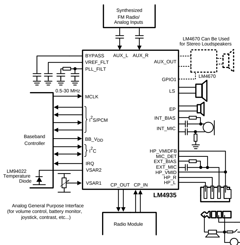
Figure 2. Example Application in Multimedia Mobile Phone
