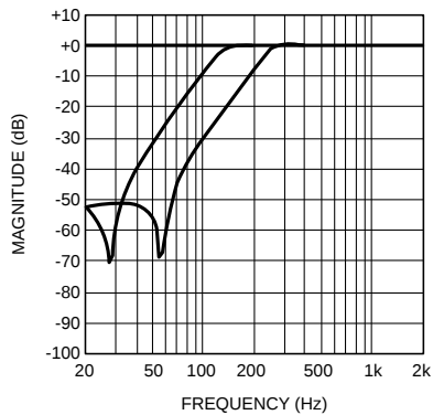
MONO ADC HPF Frequency Response f_s = 8kHz , 36dB MIC (from left to right: HPF_MODE '00', '10', '01')
