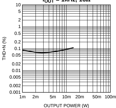
Headphone THD+N vs Output Power AV_{DD} = 3.3V , OCL 1.5V, 0dB DAC f_{OUT} = 1kHz , 16 \Omega
