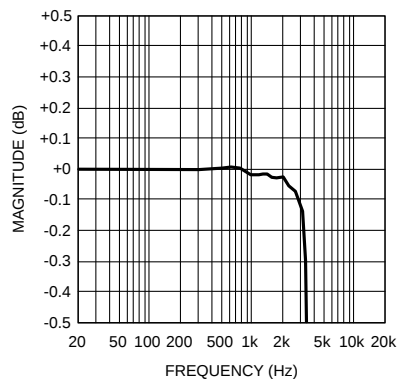
Stereo DAC Frequency Response Zoom
