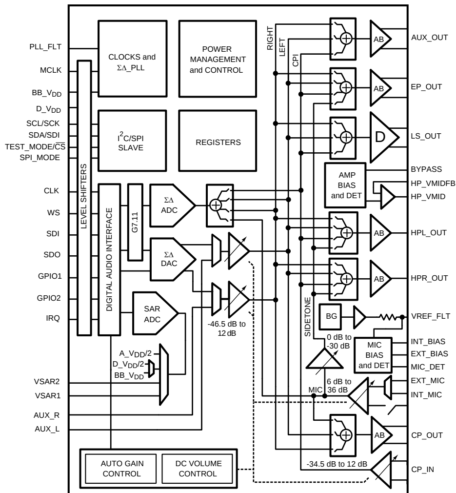
Figure 1. Conceptual Schematic
