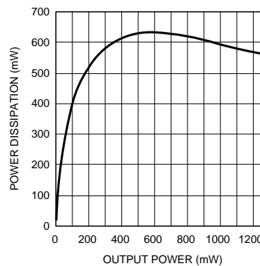
Power Dissipation vs Output Power, 2.6V, 8Ω, per channel
