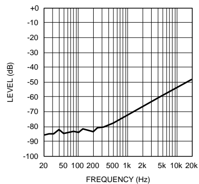
Figure 4. Input Floating
