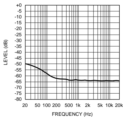
Figure 3. Input terminated with 10\Omega
