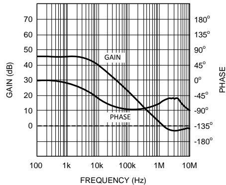
Open Loop Frequency Response, 5V
