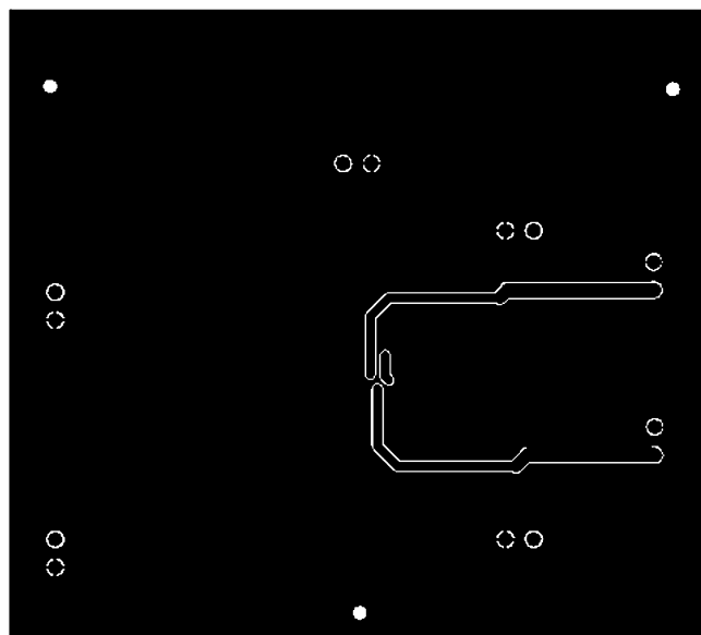
Figure 12. Recommended LLP Board Layout: Bottom Layer
