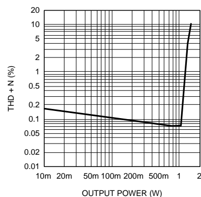
THD+N vs Power Out at V_{DD} = 5V , 8\Omega R_L , 1kHz, per channel
