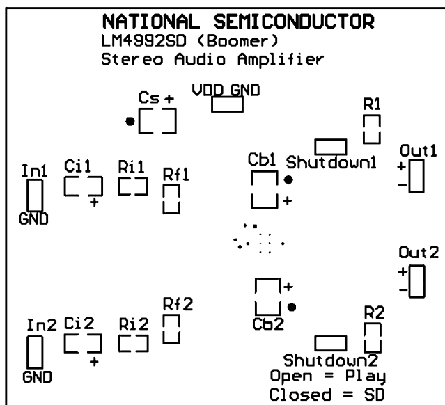
Figure 10. Recommended LLP Board Layout: Top Overlay
