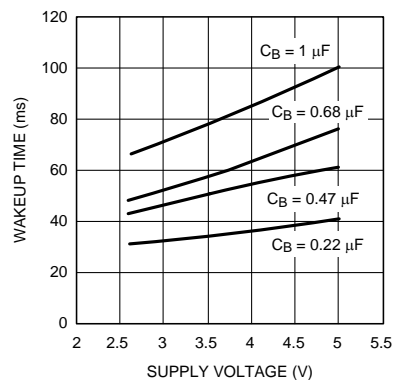
Wakeup Time vs Supply Voltage
