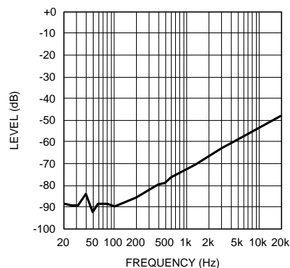
Power Supply Rejection Ratio (PSRR) vs Frequency at V_{DD} = 3.3V , 8\Omega R_L
