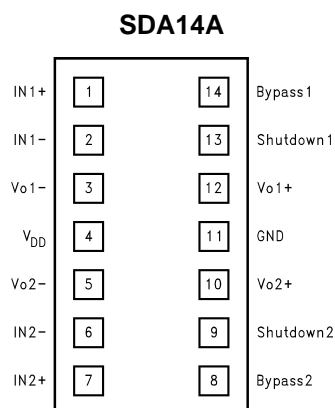
Figure 1. Top View Order Number LM4992SD See NS Package Number SDA14A
