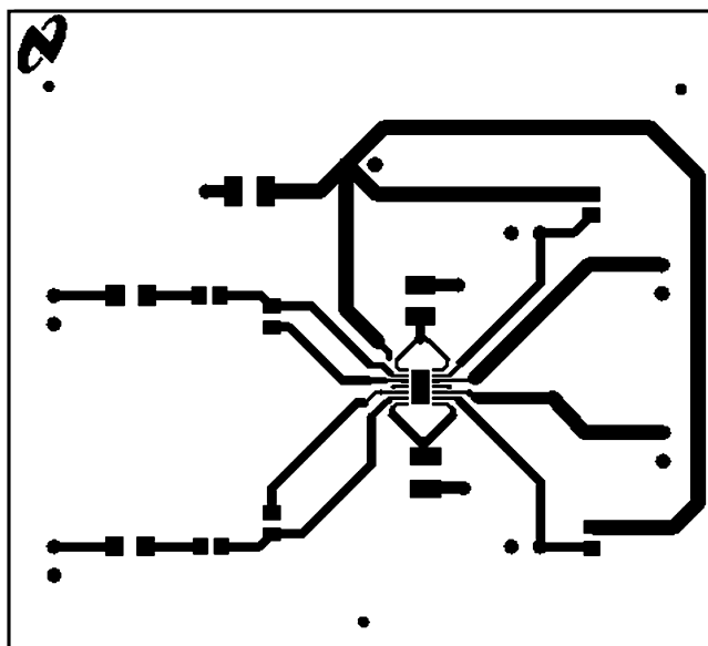
Figure 11. Recommended LLP Board Layout: Top Layer
