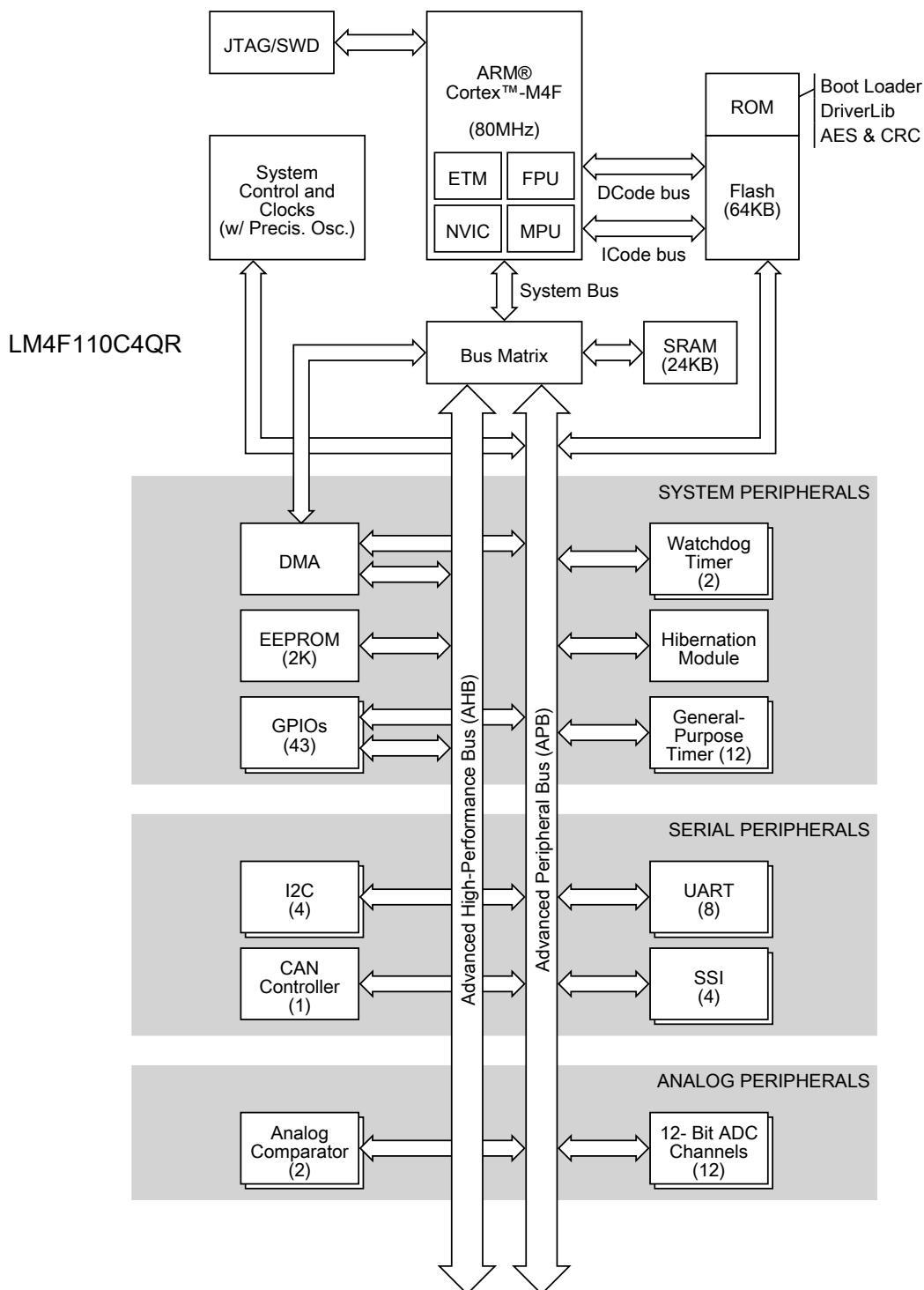
Figure 1-2. Stellaris LM4F110C4QR Microcontroller High-Level Block Diagram
