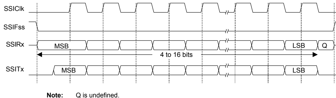
Figure 15-5. Freescale SPI Format (Continuous Transfer) with SPO=0 and SPH=0
