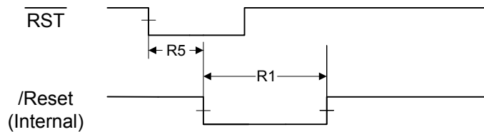
Figure 22-4. External Reset Timing (RST)
