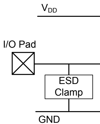
Figure 22-8. ESD Protection on Fail-Safe Pins
