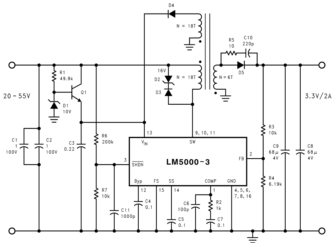
Figure 7. LM5000 Flyback Converter
