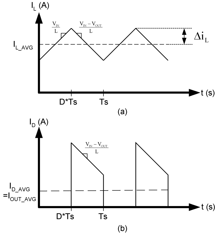
Figure 6. (a) Inductor current. (b) Diode current.
