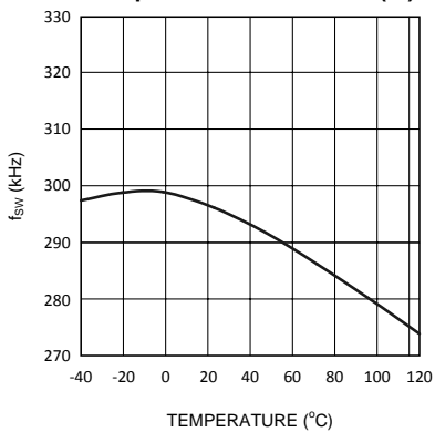
f_{SW} vs. Temperature @ FS = Low (-3)
