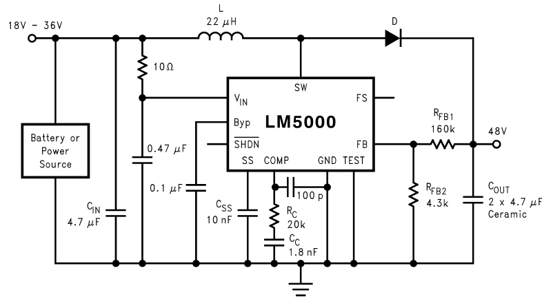
Figure 4. 700 kHz operation, 48V output
