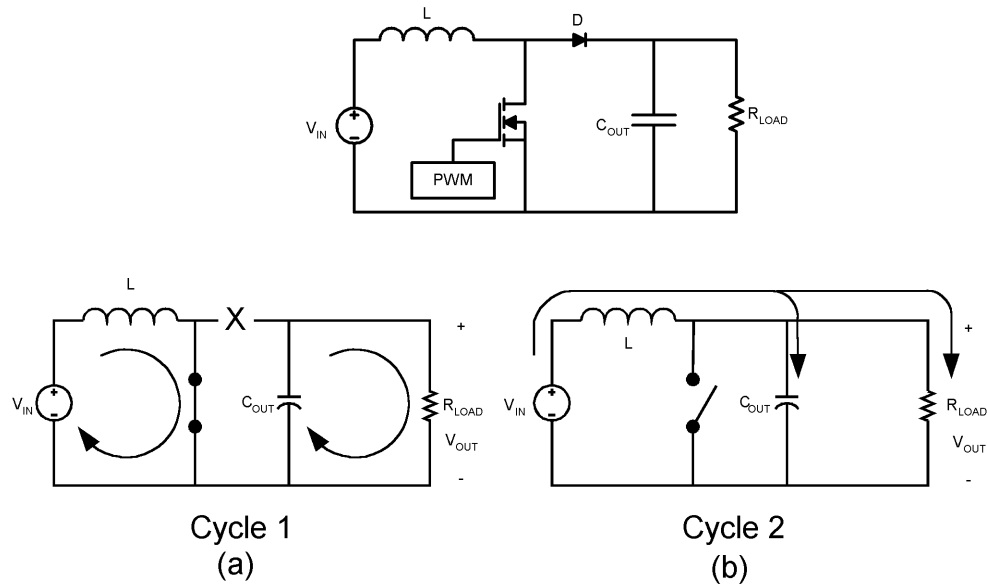
Figure 5. Simplified Boost Converter Diagram (a) First Cycle of Operation (b) Second Cycle Of Operation
