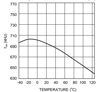
f_{SW} vs. Temperature @ FS = OPEN (-3)
