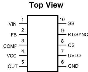
Figure 2. 10-Lead MSOP, LLP
