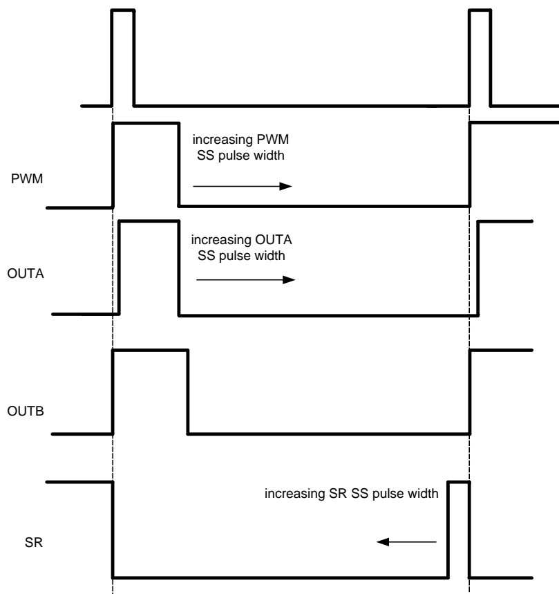
Figure 21. Soft-Start Timing
